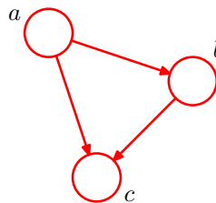
Figure 8.1 A directed graphical model representing the joint probability distribution over three variables a , b , and c , corresponding to the decomposition on the right-hand side of (8.2).
