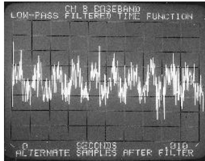
Figure 3.44 Linear averaging.
