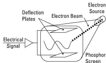
Figure 2.4 Simplified oscilloscope operation (Horizontal deflection circuits omitted for clarity).
