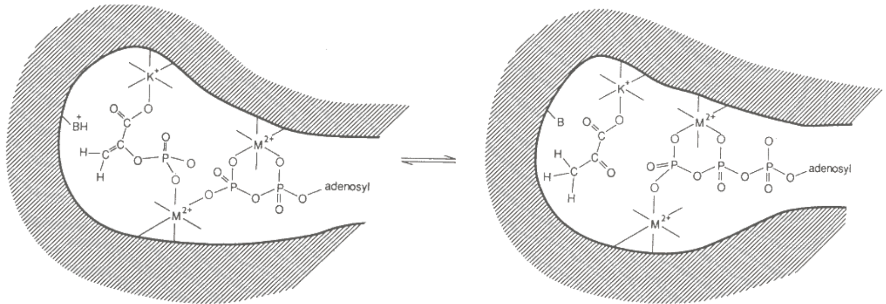
Piruvato-kinasi
