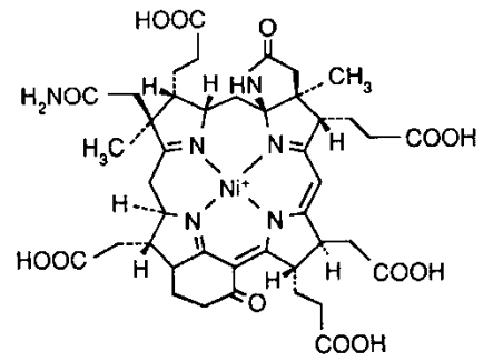
coenzyme F430
