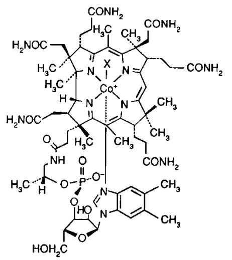
vitamin B 12 (X = CN)
