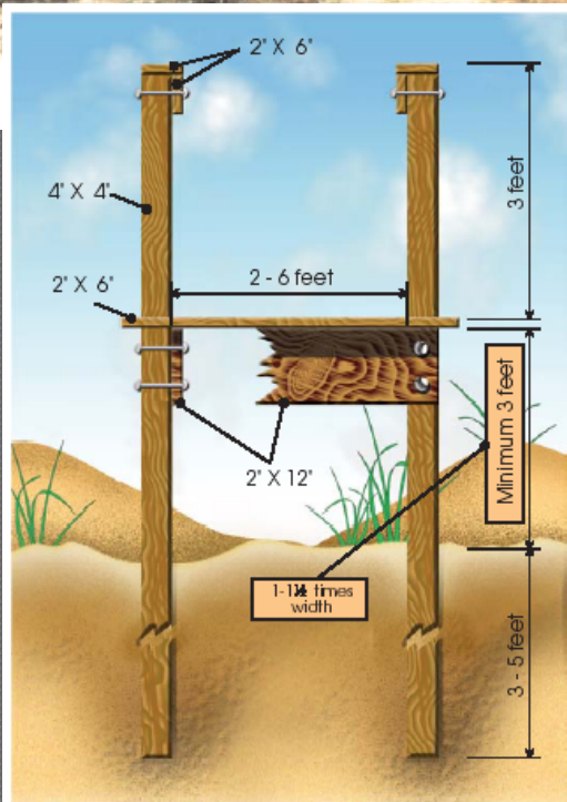
Figure 24. Construction details for a dune walkover.
