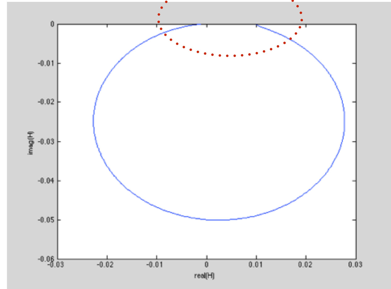
Nyquist Plot
