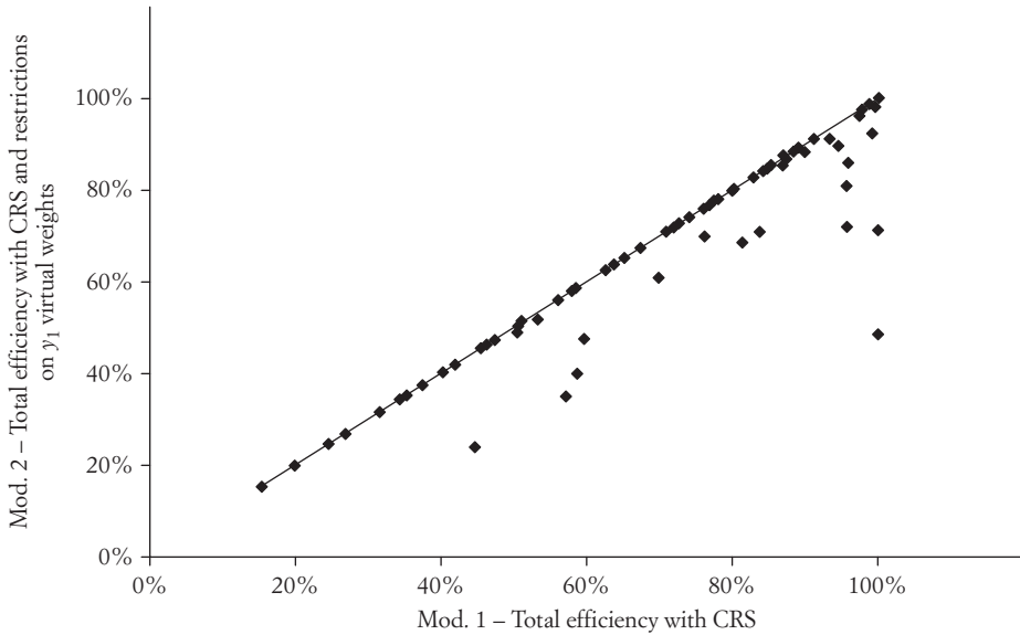
FIG. 2. Effect of a constraint on y_1 virtual weights on hospital efficiency scores.
