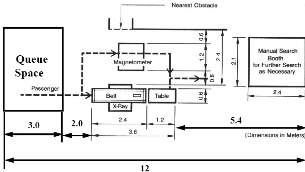
EXAMPLE OF PASSENGER SEARCH BY WALK-THROUGH MAGNETOMETER WITH HAND BAGGAGE SEARCH BY X-RAY SCANNER
