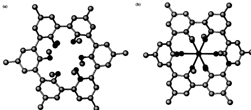
X-ray crystal structures of (a) free spherand (3.30) and (b) its \text{Li}^+ complex (after Trueblood et al. 1981).
