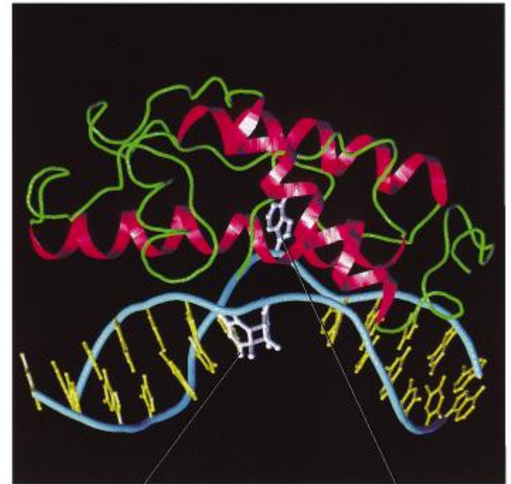
Thymine-thymine dimer
