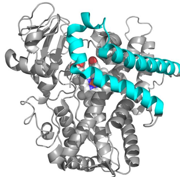
P4502B4 closed
