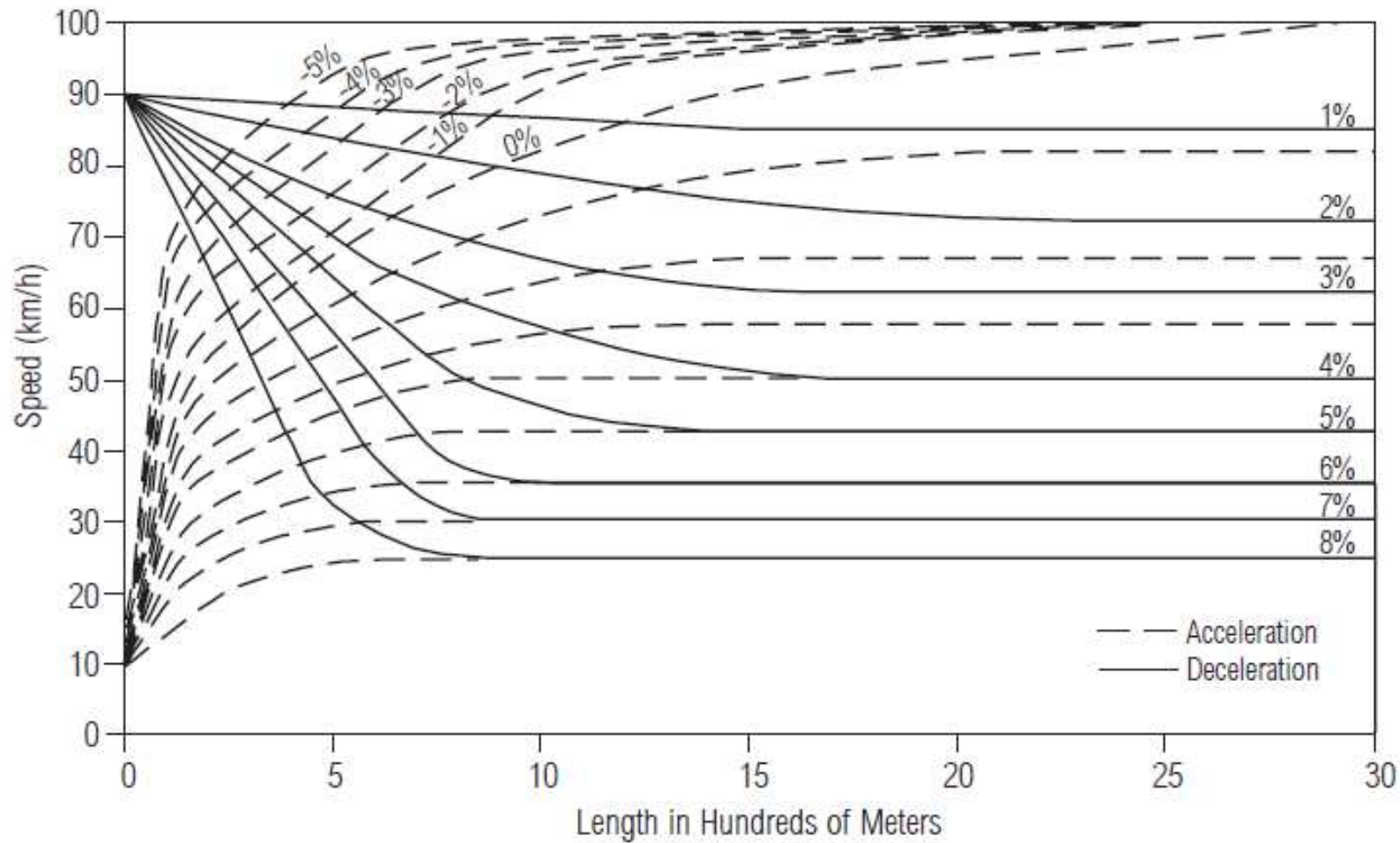
EXHIBIT A23-2. PERFORMANCE CURVES FOR TRUCKS (120 kg/kW)
