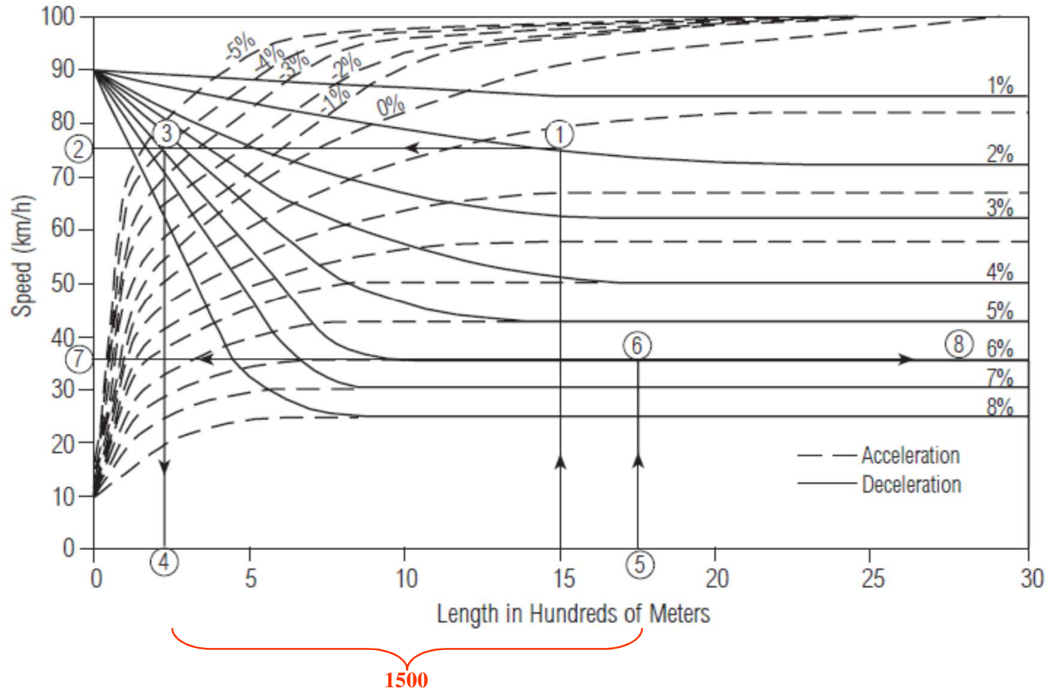
EXHIBIT A23-1. SAMPLE SOLUTION FOR COMPOSITE GRADE
