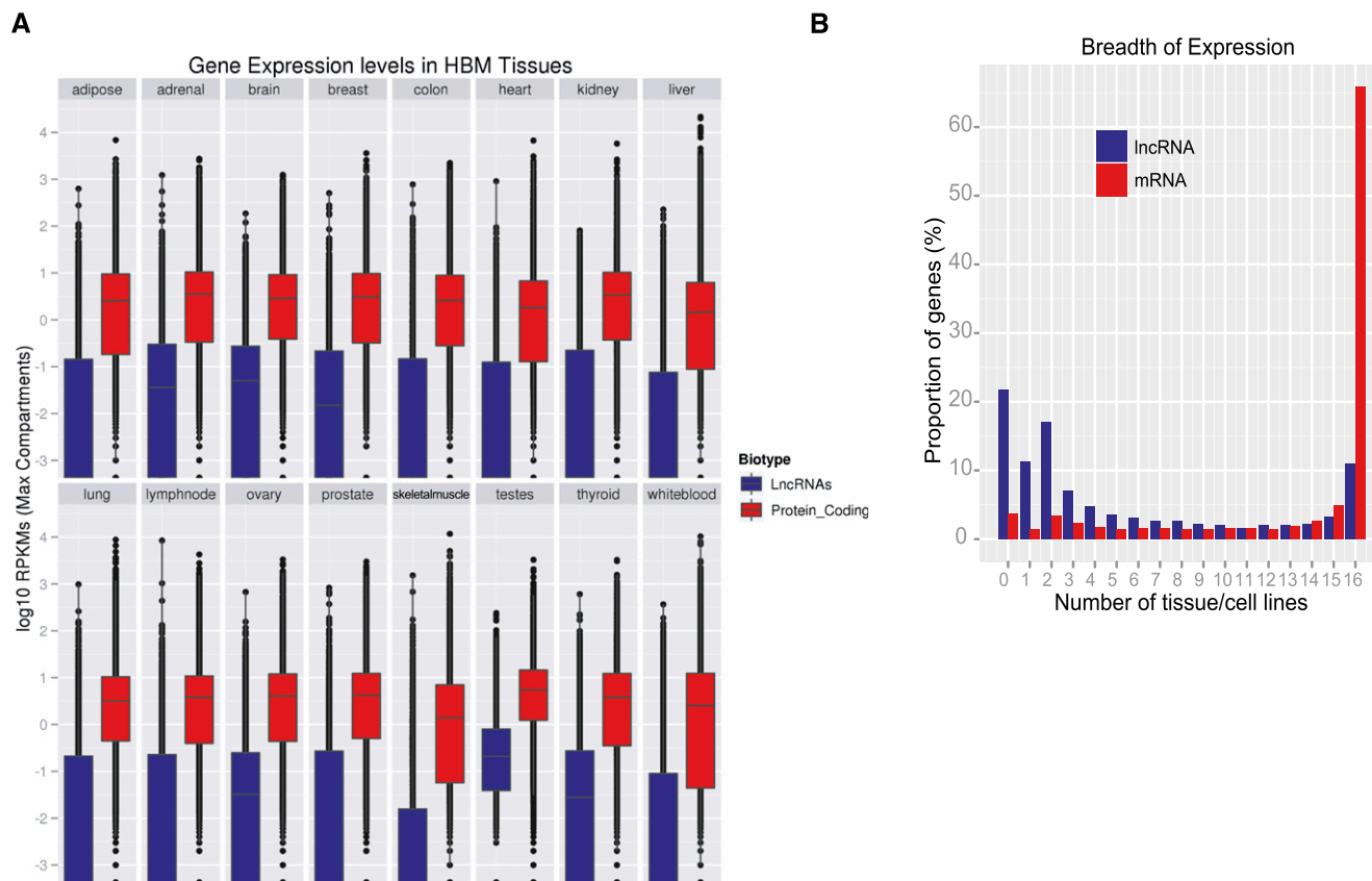
Figure 5. Characteristics of lncRNA expression in human tissues. (A) Distributions of lncRNA (blue) and protein-coding (red) transcripts' expression (log 10 RPKM) in HBM tissues. (B) Distribution of the number of HBM tissues in which lncRNA and protein-coding transcripts' are detected (RPKM > 0.1).
