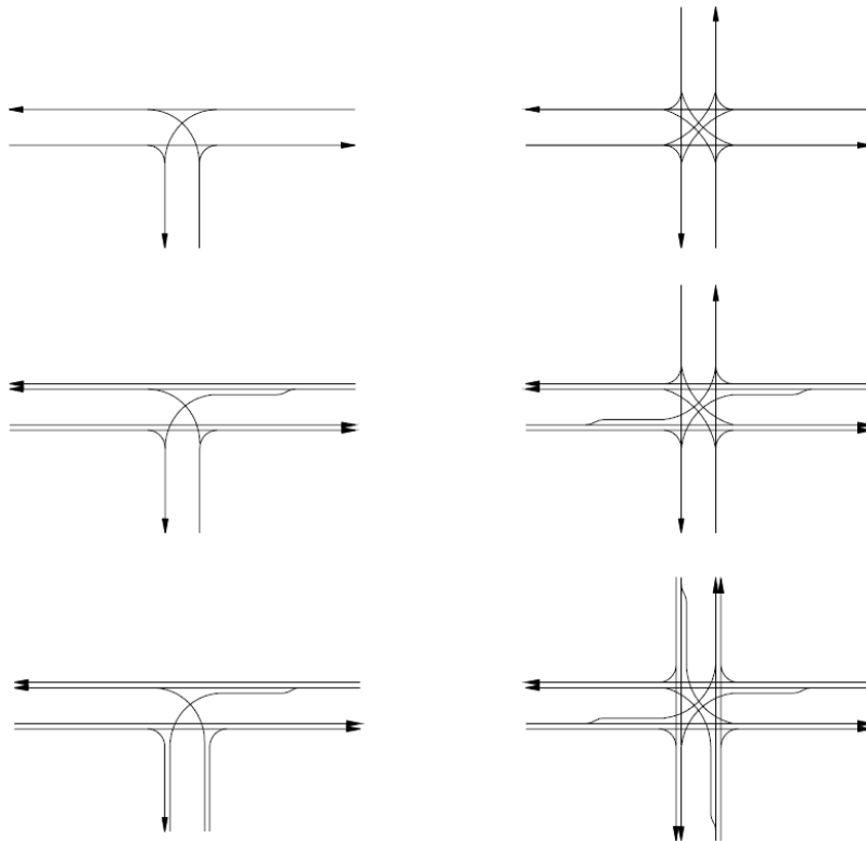
Schemi lineari
