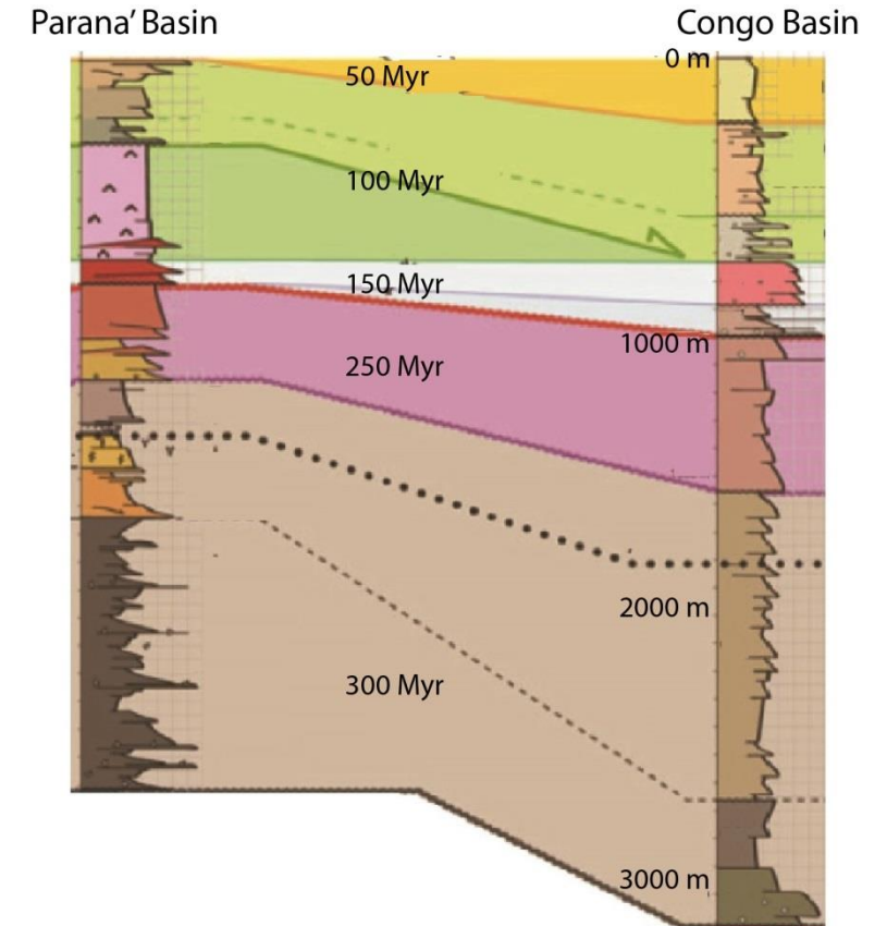
Stratigraphy Correlations
