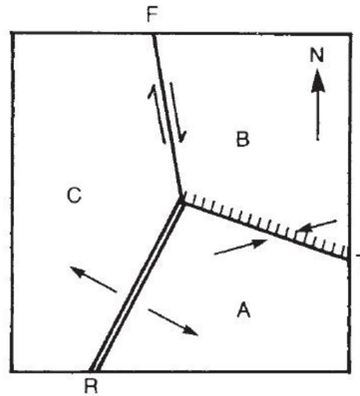
Unstable Triple Junction
