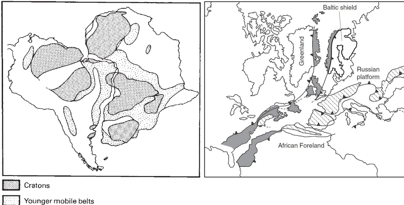
Correlation of cratons and younger mobile belts
