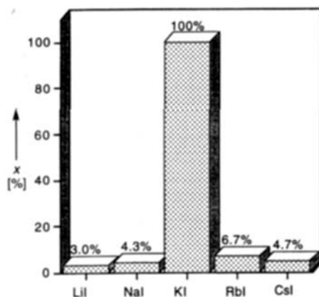
Figure 3. Uptake of alkali metal ions by 3 after treating its chloroform-methanol solution (4/1, [\mathbf{3}] = 1 \text{ mM} ) with 10 equivalents of alkali metal iodide. The complexation ratio x was determined by integration of the ^1\text{H} NMR spectra after the samples had been left to stand for 90 h. In the case of KI, equilibrium was reached within an hour.
