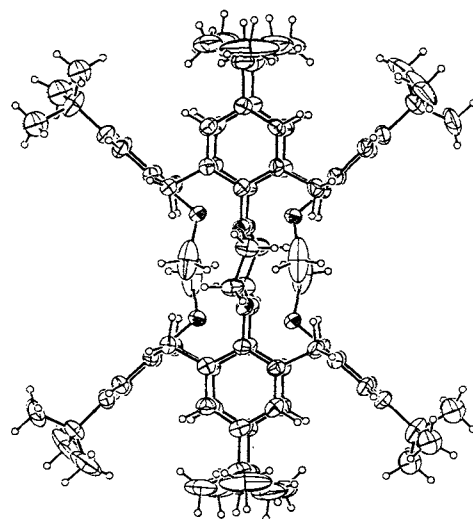
Figure 1. Crystal structure of the centrosymmetric calix[4]tube 3 in 3 \cdot 2.5 C_6H_6 , with ellipsoids at 30% probability. Hydrogen atoms are included with small arbitrary radii. The benzene solvent molecules are not shown.
