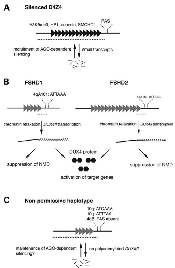
Figure 1. A DUX4-based model for FSHD, based on current data. (A) In its repressed state in somatic tissues, D4Z4 is heavily methylated (black triangles) and associated with repressive chromatin marks. Transcription occurs across the array (indicated by a dotted line) but only small transcripts are produced. siRNAs from the region reinforce silencing of the array by an Argonaute-dependent mechanism. (B) In FSHD1 and FSHD2, the array is hypomethylated (grey triangles) and loses repressive marks as a consequence of array contraction in FSHD1 or haploinsufficiency of SMCHD1 in FSHD2. A switch in transcription and splicing then leads to accumulation of DUX4fl transcripts from the most distal repeat (dotted line). These are stabilised by the PAS in permissive haplotypes and DUX4 then activates downstream targets. Transcription of the intron-containing 3' UTR of DUX4 also leads to suppression of the NMD pathway. (C) Although non-permissive haplotypes also show D4Z4 hypomethylation when contracted, the lack of a functional PAS means that DUX4fl transcripts are not stable. It is possible that the siRNA Argonaute-dependent silencing of DUX4 transcription is also maintained in this situation.
