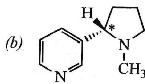
(S)-Nicotina
