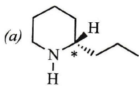
(S)-Coniina
