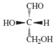
(S) -Gliceraldeide
