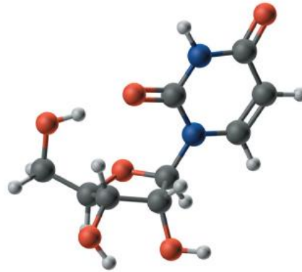
Guanina (G)
