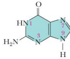
Guanina (G)
