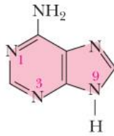
Adenina (A)
