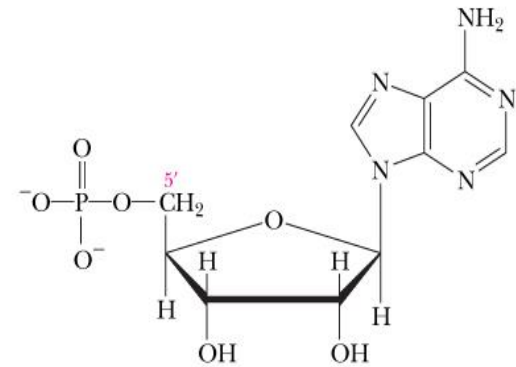
Nucleotide
