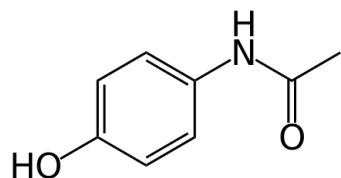
Paracetamol
