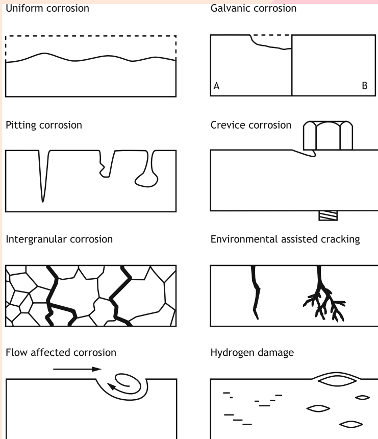
Fig. 1.3 Figure showing typical corrosion forms occurring on metals
