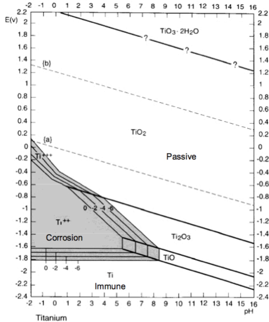
Fig. 2.1. The Pourbaix diagram for the titanium-water system [1] .
