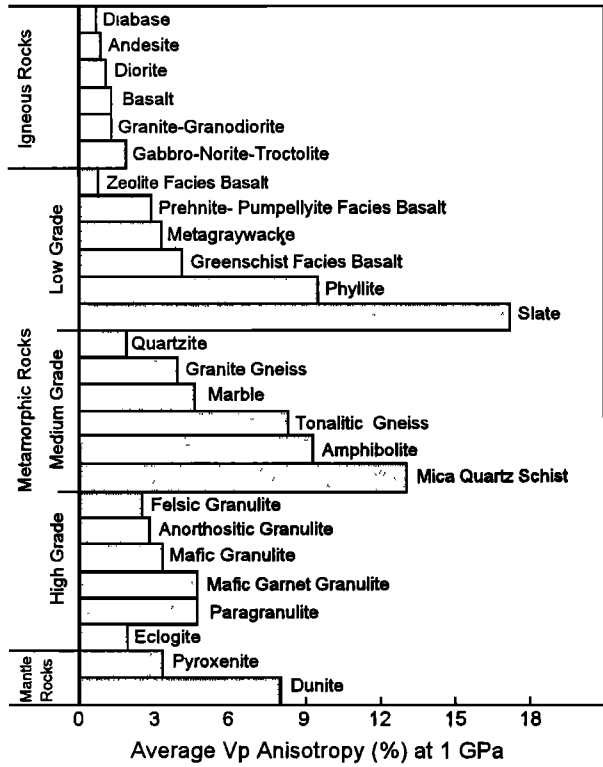
Figure 11. Average anisotropies, 100 (V_{max} - V_{min}) / V_{ave} , at pressures corresponding to 35 km depth.
