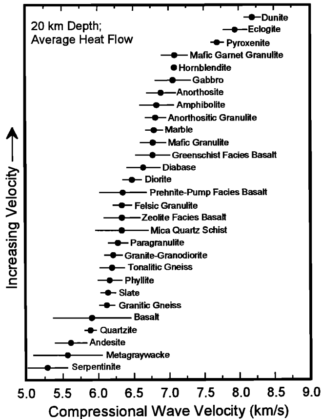
Figure 14. Average compressional wave velocities and standard deviations at 20 km depth and 309°C (average heat flow) for major rock types.
