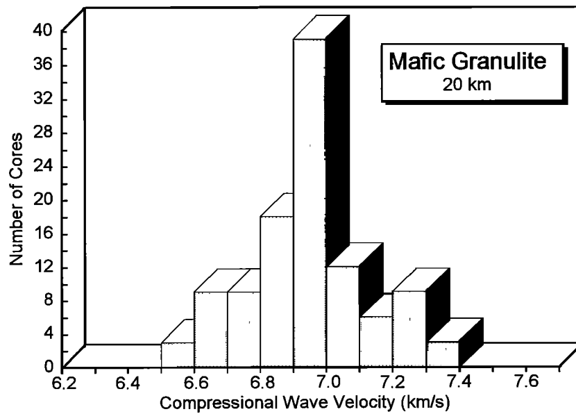
Figure 10. Mafic granulite velocities at pressures corresponding to 20 km depth.
