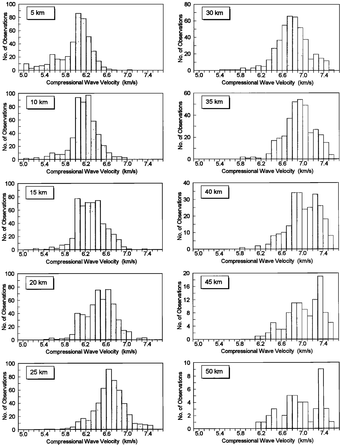
Figure 5. Histograms of crustal velocity at 5-km depth intervals. Locations of data are shown in Figure 1. Data have not been sorted by geologic or tectonic setting or crustal age. Shallow crustal velocities less than 5.0 km/s, corresponding to sedimentary rocks, and sub-Moho velocities greater than 7.5 km/s have been excluded.
