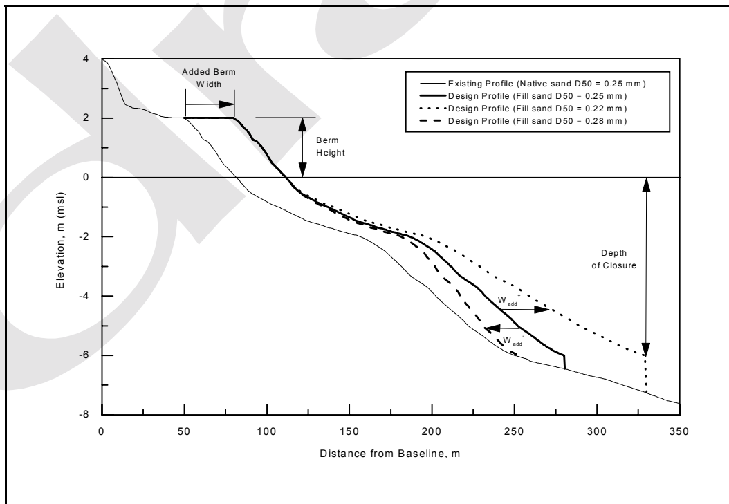
Figure V-4-17. Design profiles for different fill sand sizes
