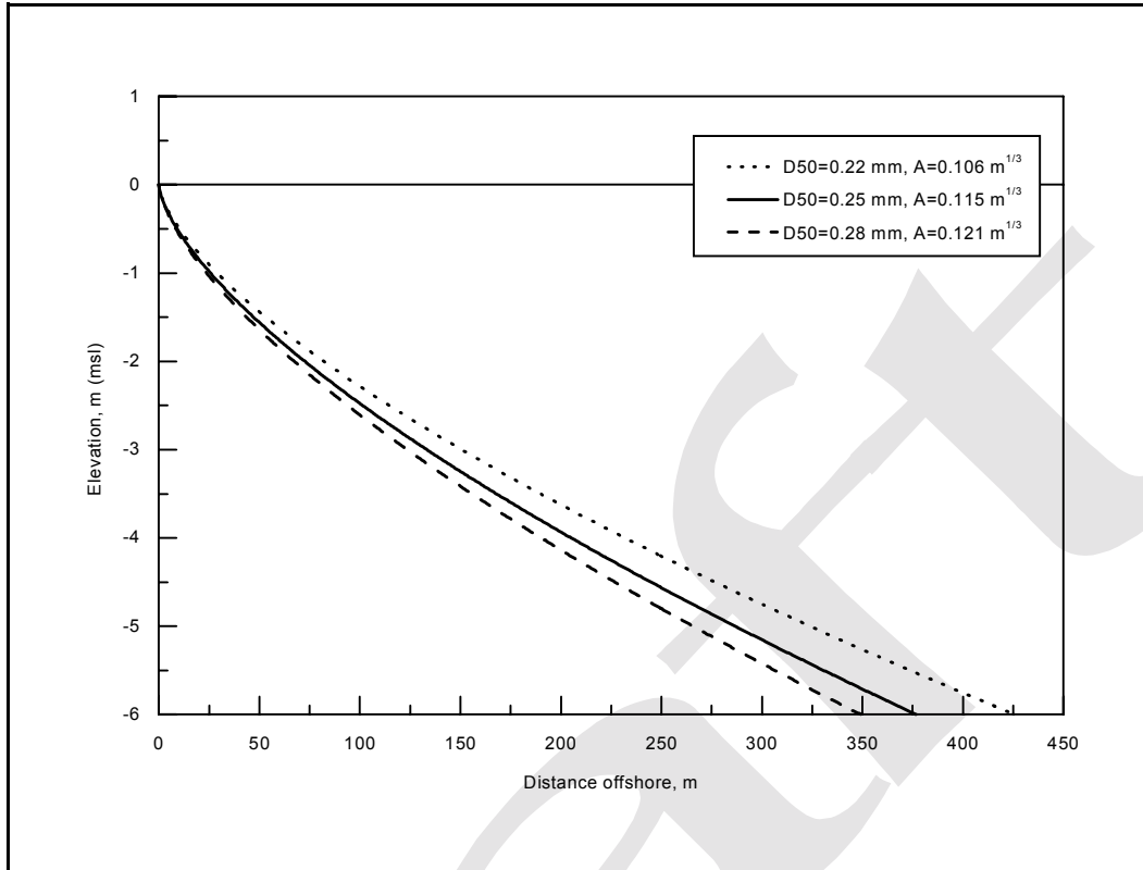
Figure V-4-16. Theoretical equilibrium profile shapes for different sand grain sizes
