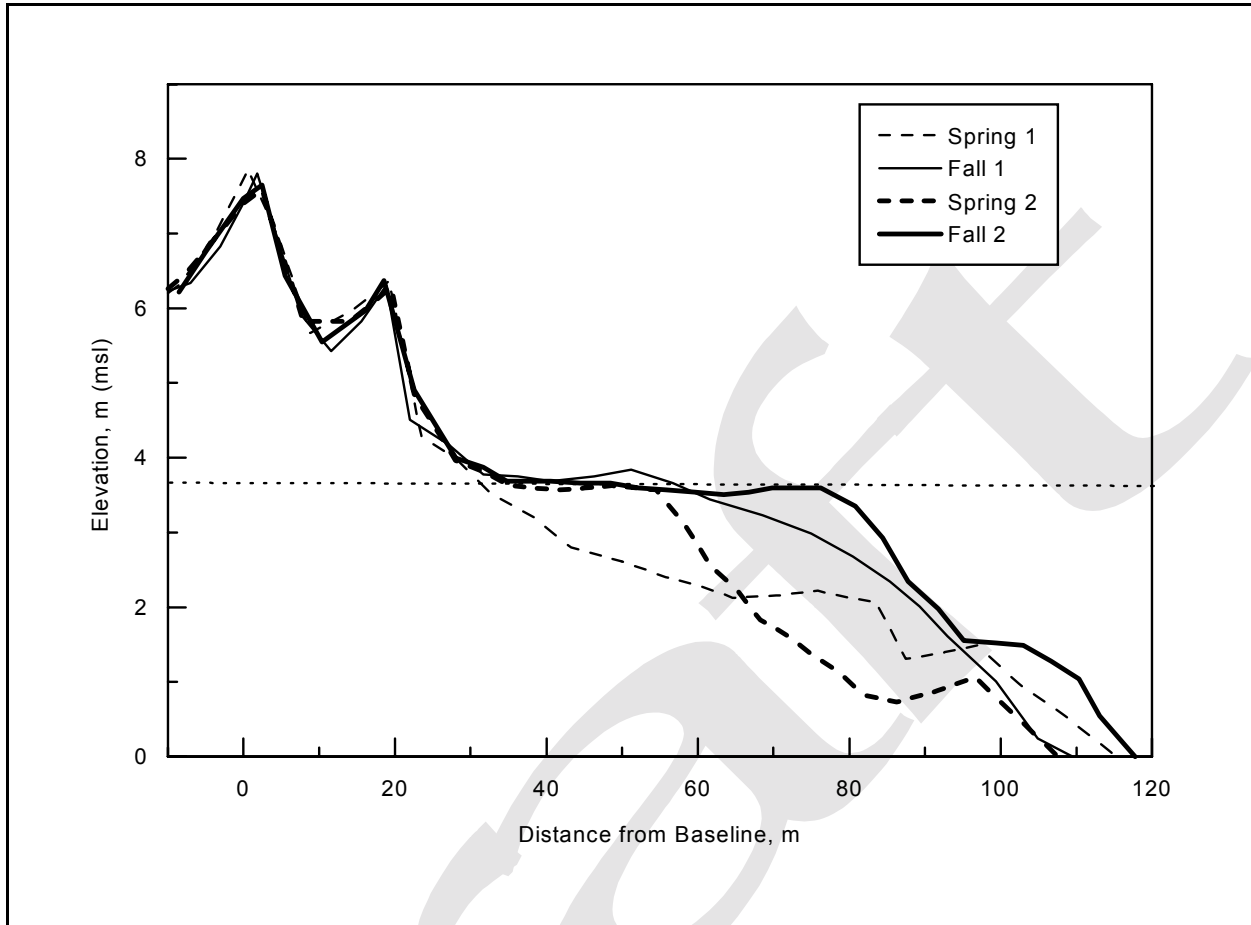
Figure V-4-10. Seasonal variation of a beach berm
