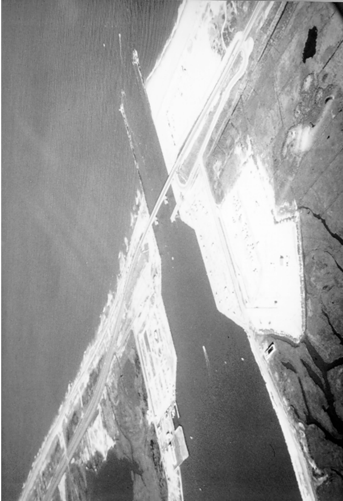
Figure III-2-1. Impoundment of longshore sediment transport at Indian River Inlet, Delaware
