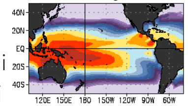
January-March Mean Ocean Temperatures (°C)
