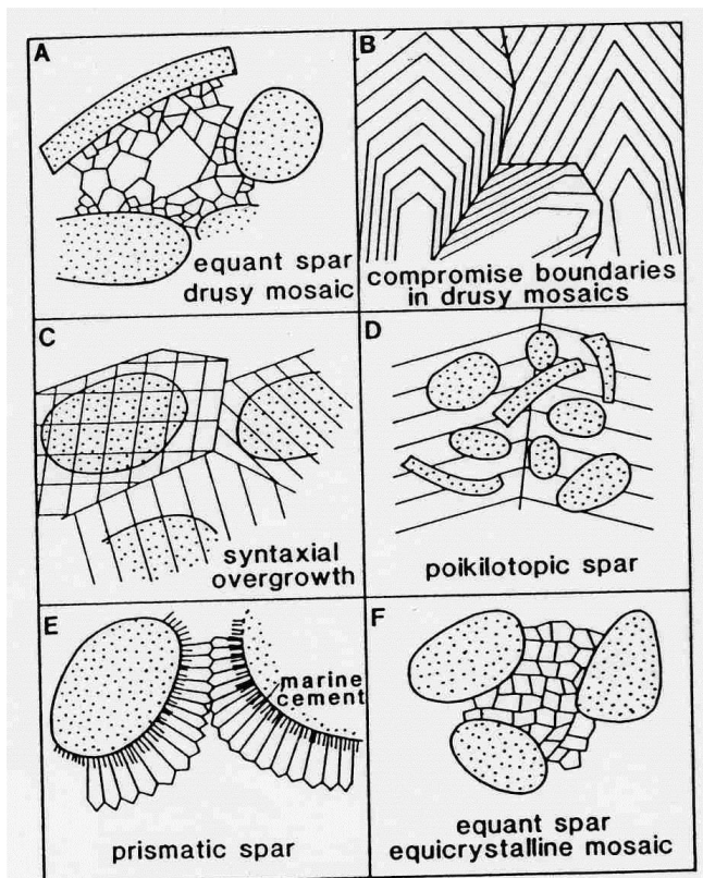
Fig. 7.32 Calcite spar: sketches illustrating the common types.
