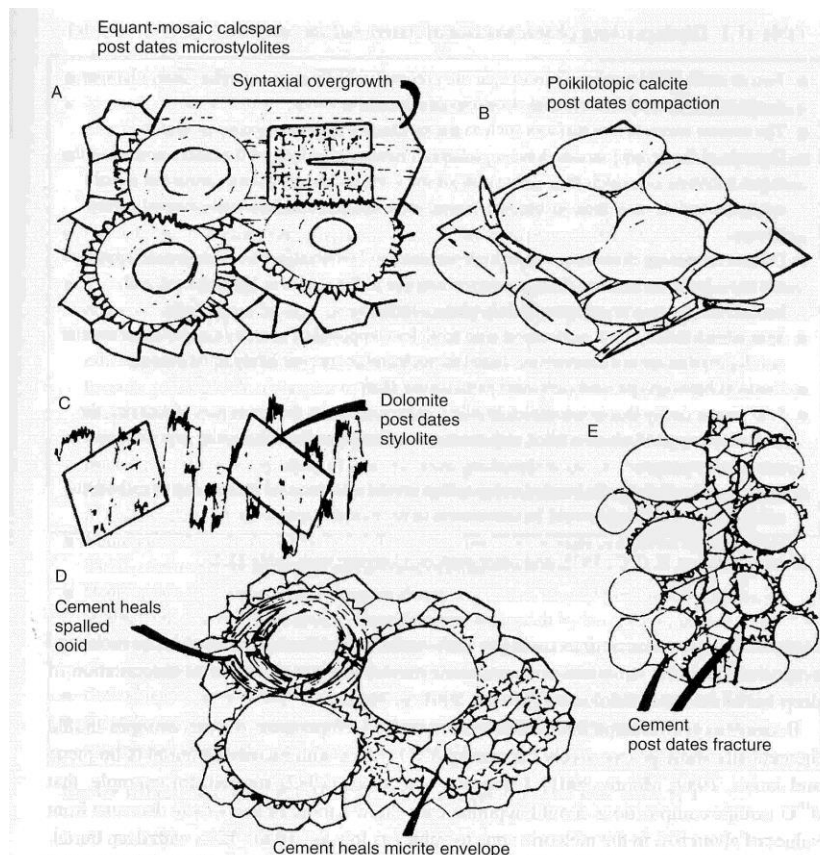
Figure 11.14 Examples of criteria that suggest late-burial cementation. A. Syntaxial overgrowth encloses microstylolites formed during a preceding stage of chemical compaction. B. Calcite poikilotopically encompasses grains packed and broken during physical compaction. C. Cement crystals cut across stylolites formed during chemical compaction. D. Ooids or micrite envelopes broken during compaction are healed by cement. E. Cement fills late-stage tectonic fractures. (From
