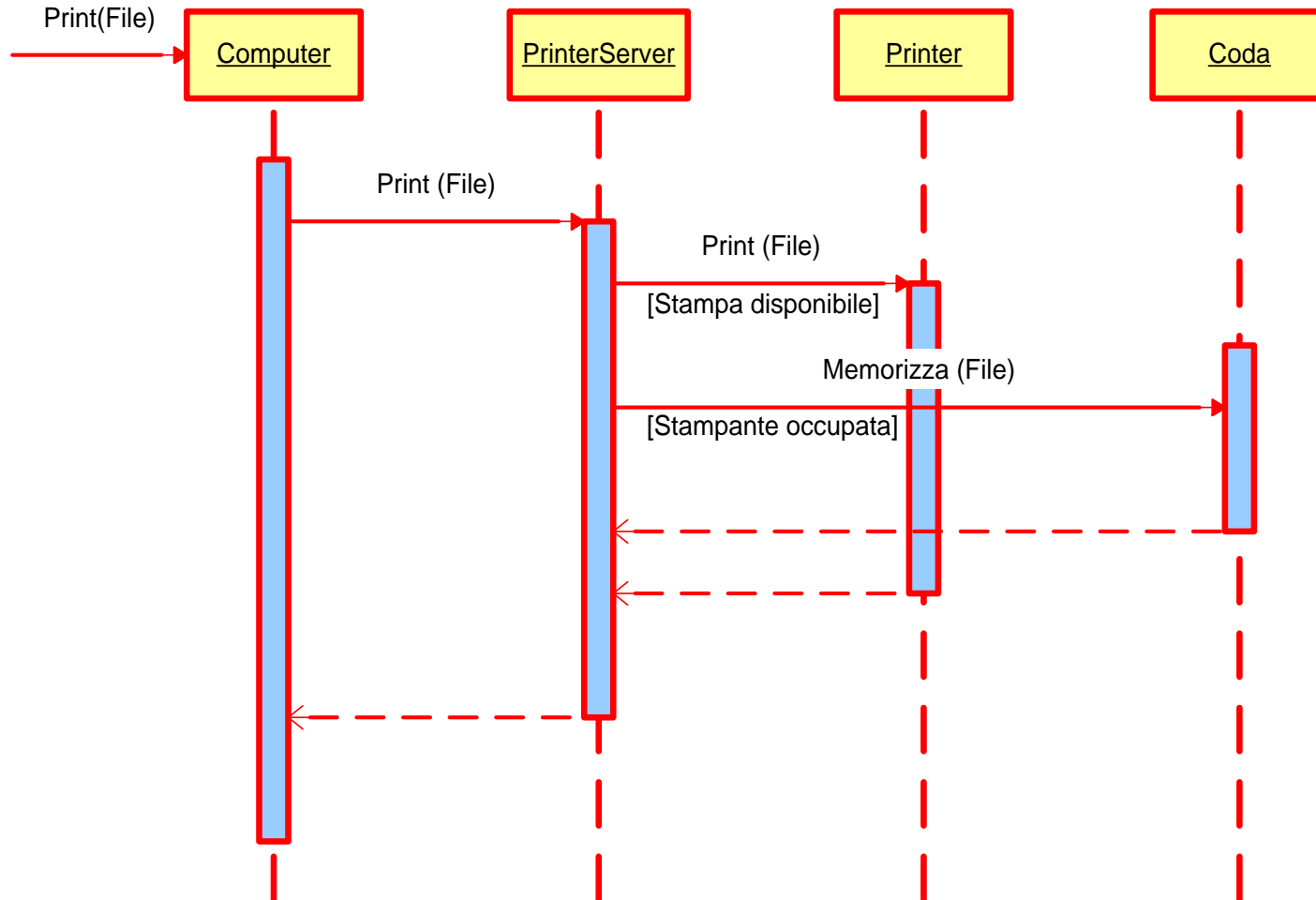
Sequence Diagram
