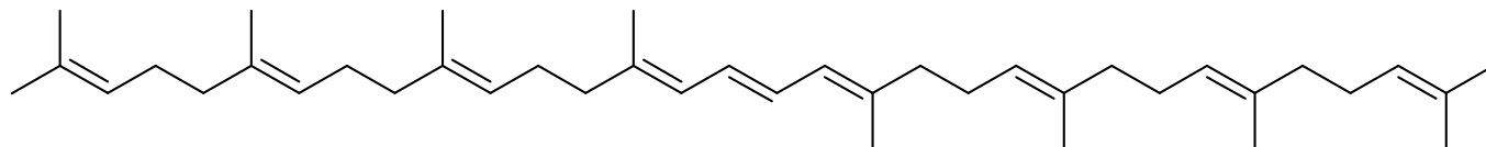
FITOENE
