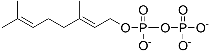
GeraniilPP
