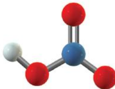
\text{HNO}_3 , Acido nitrico
