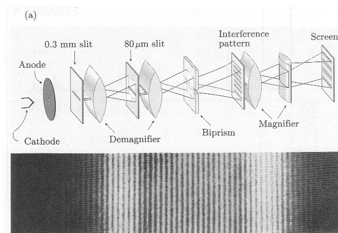
FIGURE 14.7 Double-slit interference of electrons: (a) apparatus; (b) interference pattern. Taken from H. Düker, Z. Naturforsch. 10a, 256 (1955) with permission of the publisher
