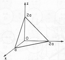
Fig. 4 A (211)-crystal plane.
