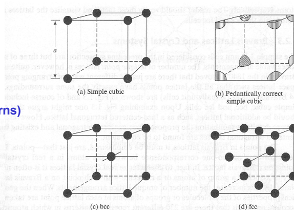
Figure 1.2 Simple three-dimensional unit cells. (a) Simple cubic unit cell. (b) Pedantically correct simple cubic unit cell including only the fractional portion (1/8) of each corner atom actually within the cell cube. (c) Body-centered cubic unit cell. (d) Face-centered cubic unit cell (After Pierret. [3] )
