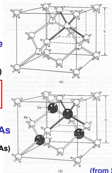
Fig. 3 (a) Diamond lattice. (b) Zincblende lattice.
