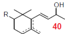
R=H, R'=Me trans - \alpha -irone R=Me, R'=H cis - \alpha -irone
