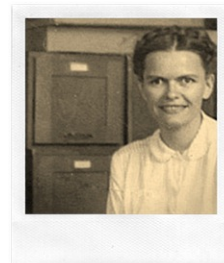
Julia Robinson, 1919–1985
