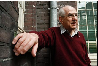
Hilary Putnam, 1926–2016
