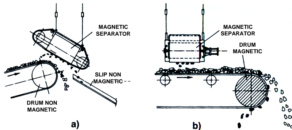
Magnetic separators
