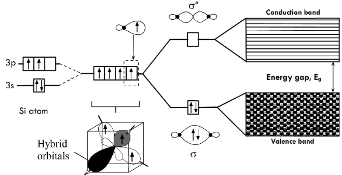
Figure 4: Formation of energy bands in Si. (a) Si atom with 4 electrons in outer shell form (b) 4 sp^3 hybrid orbitals. (c) The hybrid orbitals form \sigma and \sigma^* orbitals. (d) These orbitals overlap in a solid to form the valence and conduction band. Adapted from Principles of Electronic Materials - S.O. Kasap.
