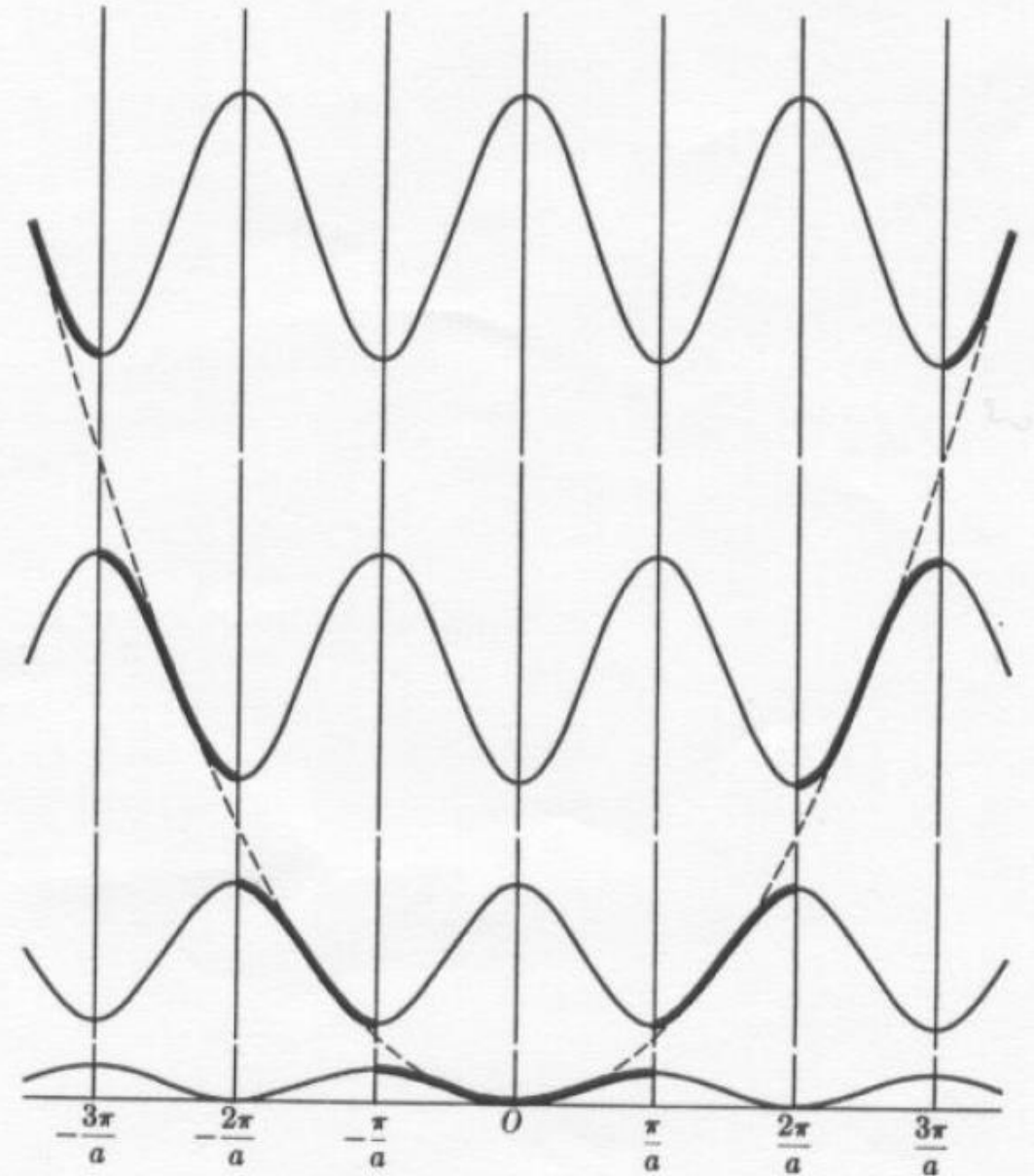
Fig. 6-33. Allowed energies in the tight-binding approximation.
