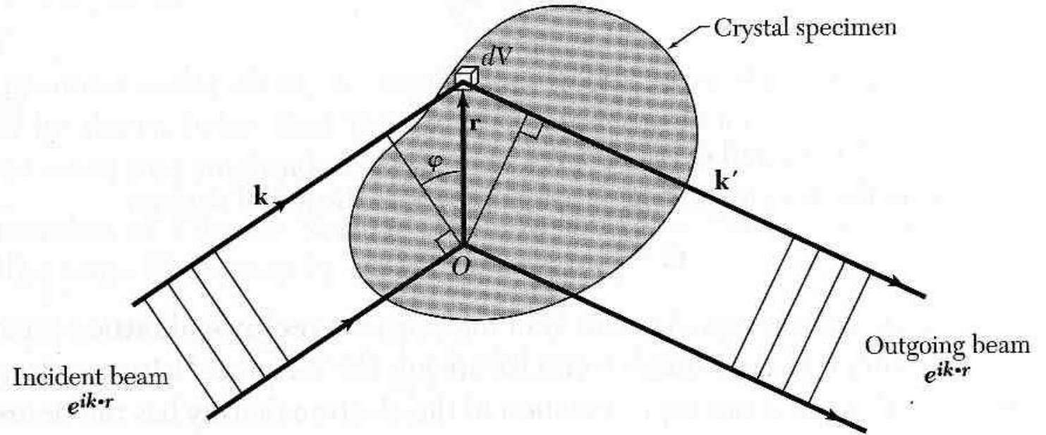
Figure 6 The difference in path length of the incident wave \mathbf{k} at the points O , \mathbf{r} is r \sin \varphi , and the difference in phase angle is (2\pi r \sin \varphi)/\lambda , which is equal to \mathbf{k} \cdot \mathbf{r} . For the diffracted wave the difference in phase angle is -\mathbf{k}' \cdot \mathbf{r} . The total difference in phase angle is (\mathbf{k} - \mathbf{k}') \cdot \mathbf{r} , and the wave scattered from dV at \mathbf{r} has the phase factor \exp[i(\mathbf{k} - \mathbf{k}') \cdot \mathbf{r}] relative to the wave scattered from a volume element at the origin O .
