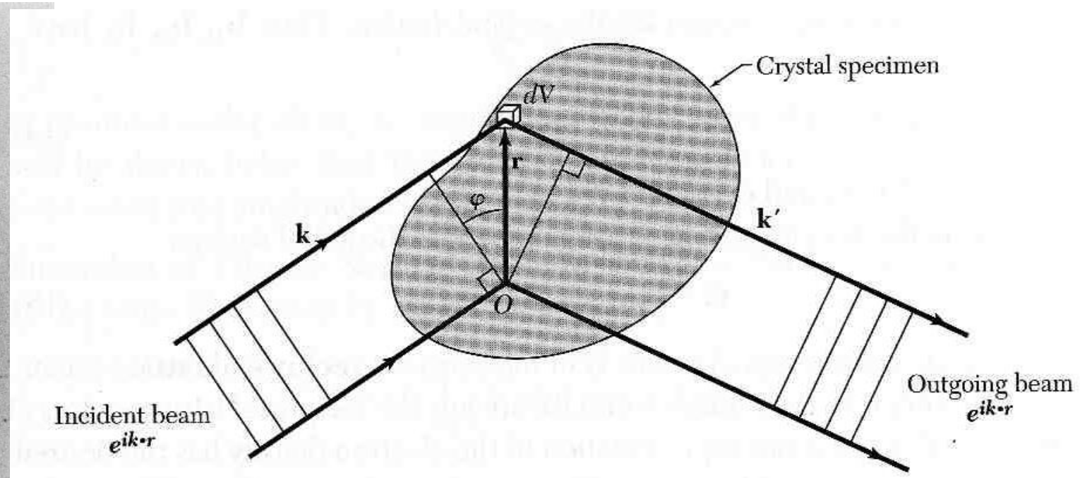
Figure 6 The difference in path length of the incident wave \mathbf{k} at the points O , \mathbf{r} is r \sin \varphi , and the difference in phase angle is (2\pi r \sin \varphi)/\lambda , which is equal to \mathbf{k} \cdot \mathbf{r} . For the diffracted wave the difference in phase angle is -\mathbf{k}' \cdot \mathbf{r} . The total difference in phase angle is (\mathbf{k} - \mathbf{k}') \cdot \mathbf{r} , and the wave scattered from dV at \mathbf{r} has the phase factor \exp[i(\mathbf{k} - \mathbf{k}') \cdot \mathbf{r}] relative to the wave scattered from a volume element at the origin O .
