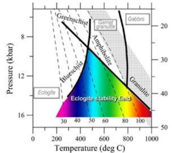
Artemieva and Meissner, 2012, Tectonophysics 530-531
