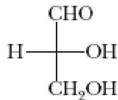
D-Gliceraldeide
