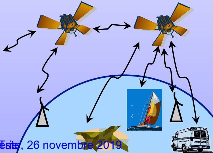
cross-link in communication satellite system
