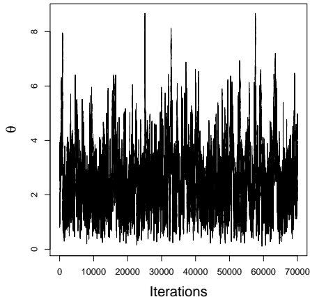
Markov chain
