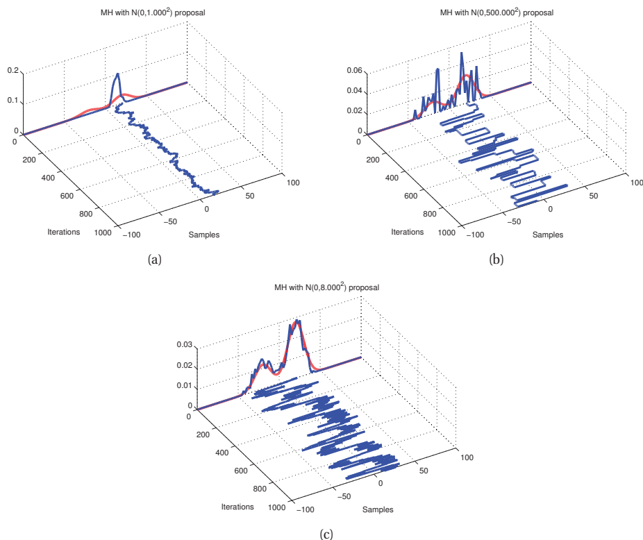
Figure 24.7 An example of the Metropolis Hastings algorithm for sampling from a mixture of two 1D Gaussians ( \boldsymbol{\mu} = (-20, 20) , \boldsymbol{\pi} = (0.3, 0.7) , \boldsymbol{\sigma} = (100, 100) ), using a Gaussian proposal with variances of v \in \{1, 500, 8\} . (a) When v = 1 , the chain gets trapped near the starting state and fails to sample from the mode at \mu = -20 . (b) When v = 500 , the chain is very “sticky”, so its effective sample size is low (as reflected by the rough histogram approximation at the end). (c) Using a variance of v = 8 is just right and leads to a good approximation of the true distribution (shown in red). Figure generated by mcmcGmmDemo . Based on code by Christophe Andrieu and Nando de Freitas.
