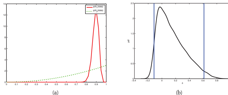
Figure 5.5 (a) Exact posteriors p(\theta_i|\mathcal{D}_i) . (b) Monte Carlo approximation to p(\delta|\mathcal{D}) . We use kernel density estimation to get a smooth plot. The vertical lines enclose the 95% central interval. Figure generated by amazonSellerDemo ,
