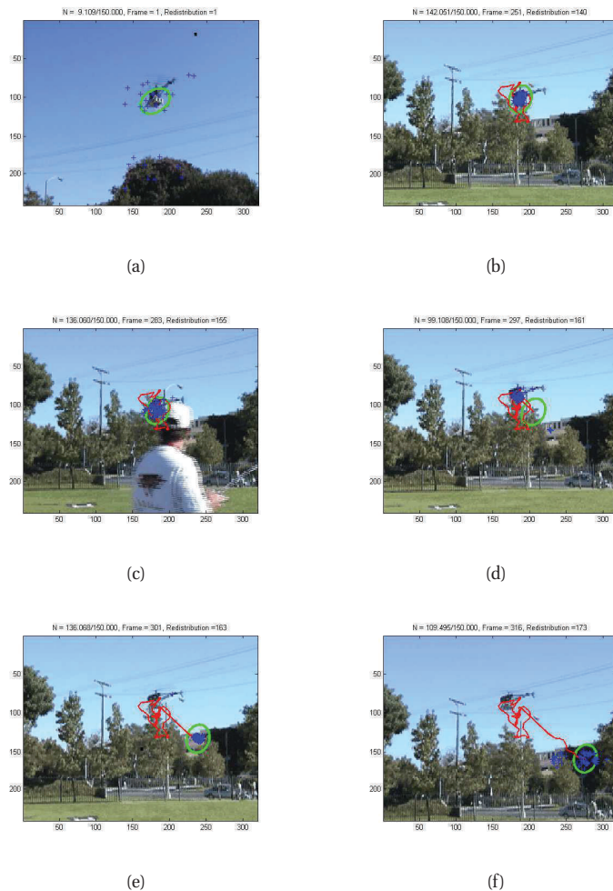
Figure 23.6 Example of particle filtering applied to visual object tracking, based on color histograms. (a-c) successful tracking: green ellipse is on top of the helicopter. (d-f): tracker gets distracted by gray clutter in the background. See text for details. Figure generated by pfColorTrackerDemo , written by Sebastien Paris.
