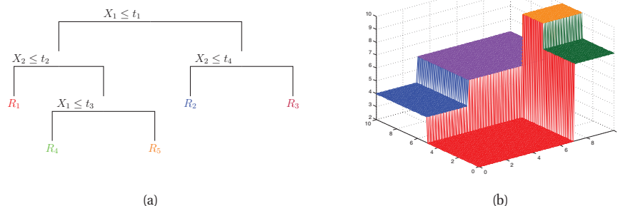
Figure 16.1 A simple regression tree on two inputs. Based on Figure 9.2 of (Hastie et al. 2009). Figure generated by regtreeSurfaceDemo .
