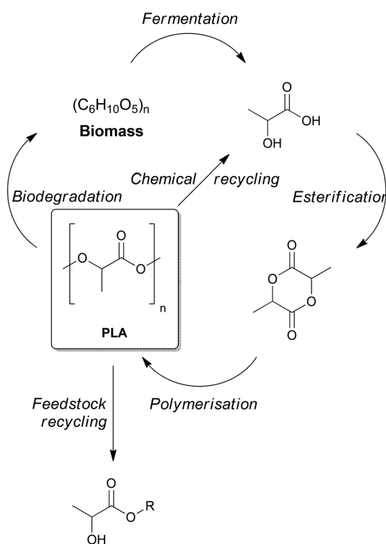
Scheme 6 Chemical recycling options for PLA.
