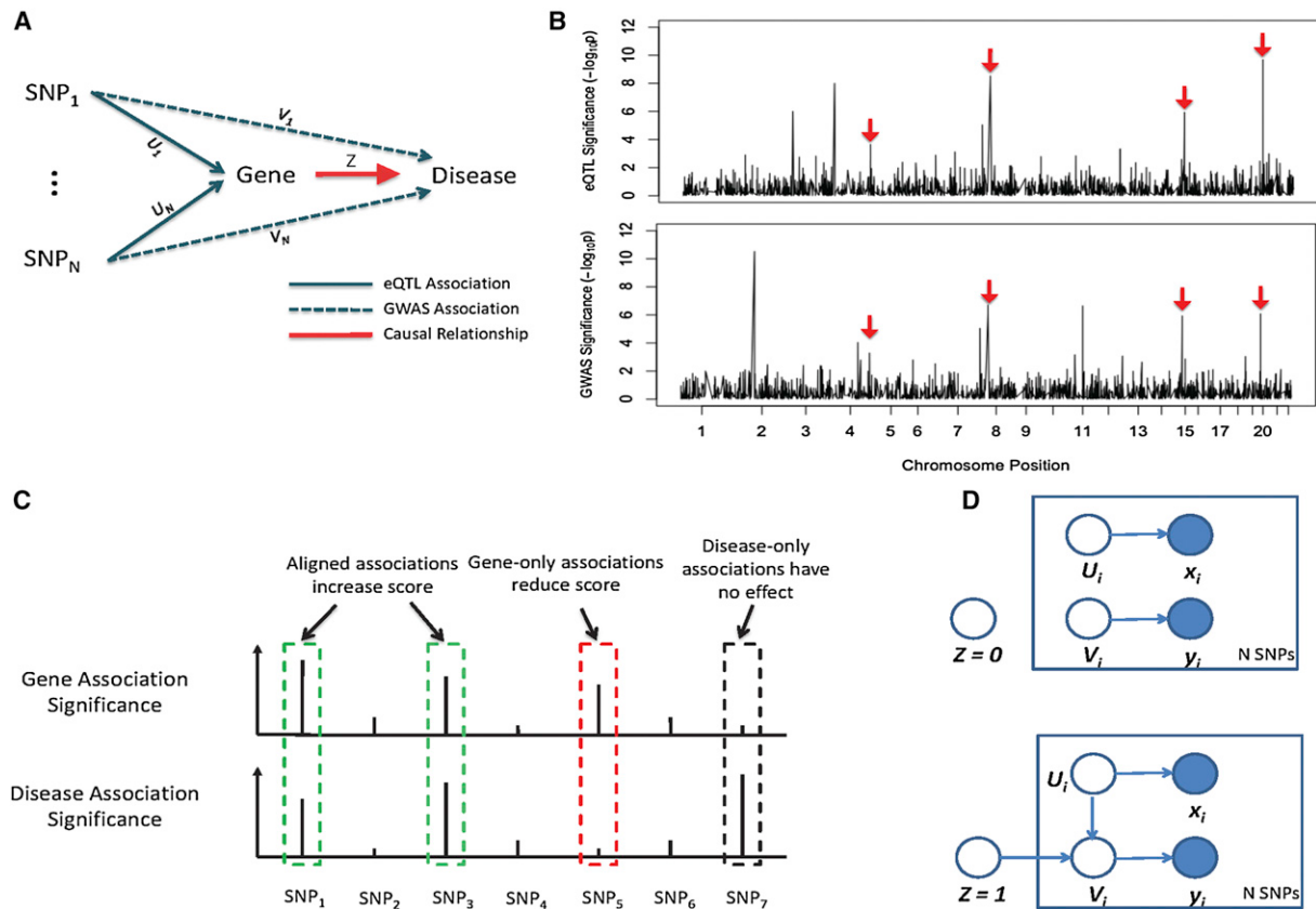
Figure 1. The Sherlock Algorithm: Matching Genetic Signatures of Gene Expression Traits to that of the Disease to Identify Gene-Disease Associations
