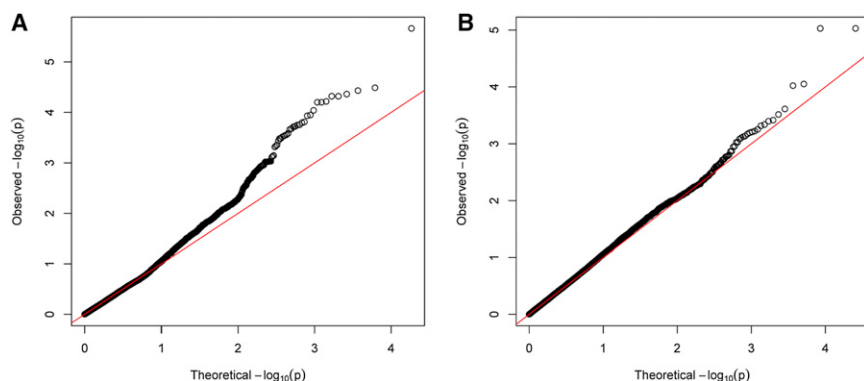
Figure 2. Quantile-Quantile Plots of the p Values at the Log. Scale of All Genes Calculated by Sherlock
