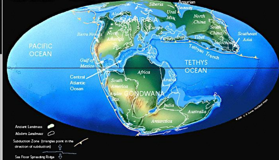
Late Jurassic 152 Ma
