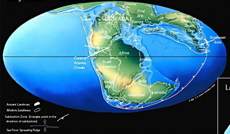
Early Jurassic 195 Ma
