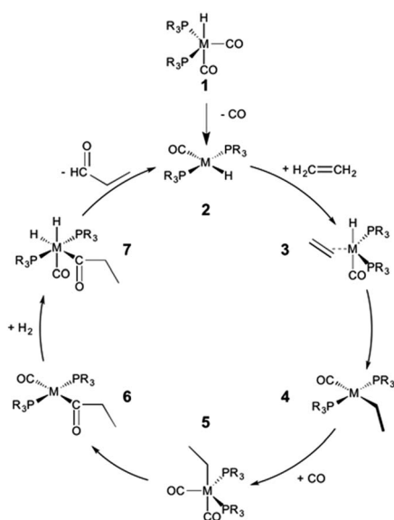
Fig. 2 Mechanism for the Rh-catalyzed hydroformylation of an olefin. M = Rh, R = Ph.
