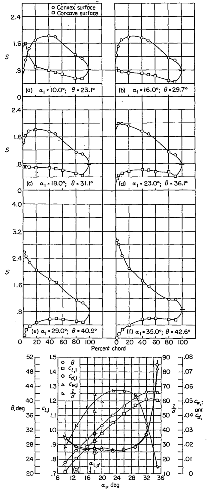
(g) Section characteristics; flagged symbol indicates leading-edge roughness.
