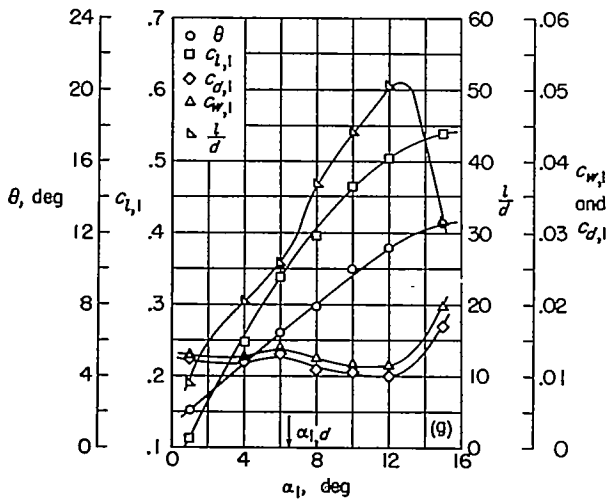
(g) Section characteristics.
