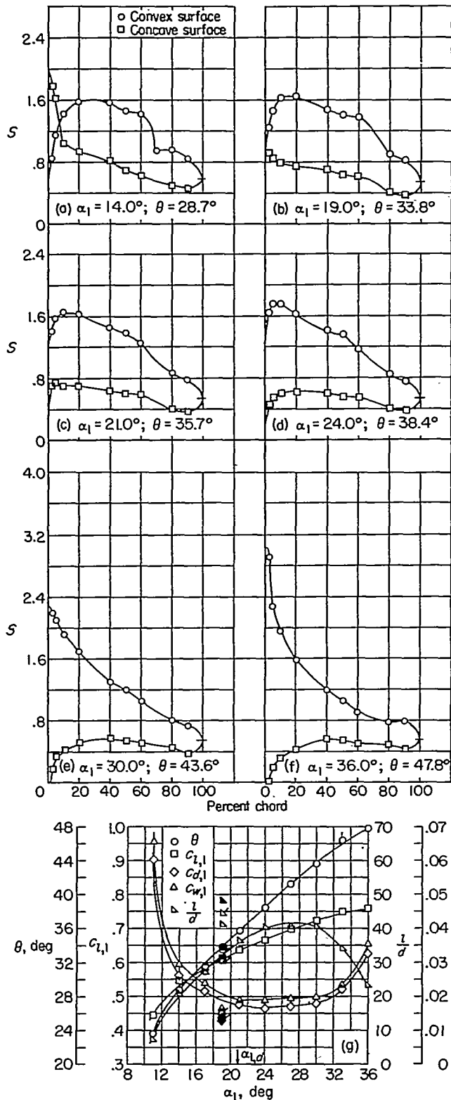
(g) Section characteristics; flagged symbol indicates leading-edge roughness; solid symbol indicates high Reynolds number.
