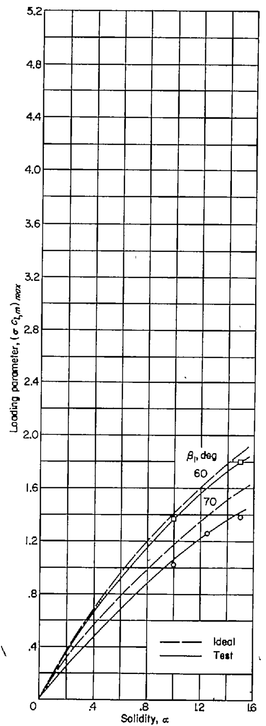
FIGURE 89.—Variation of the limit loading parameter, (\sigma c_{l,m})_{max} with solidity for inlet angles of 60^\circ and 70^\circ .
