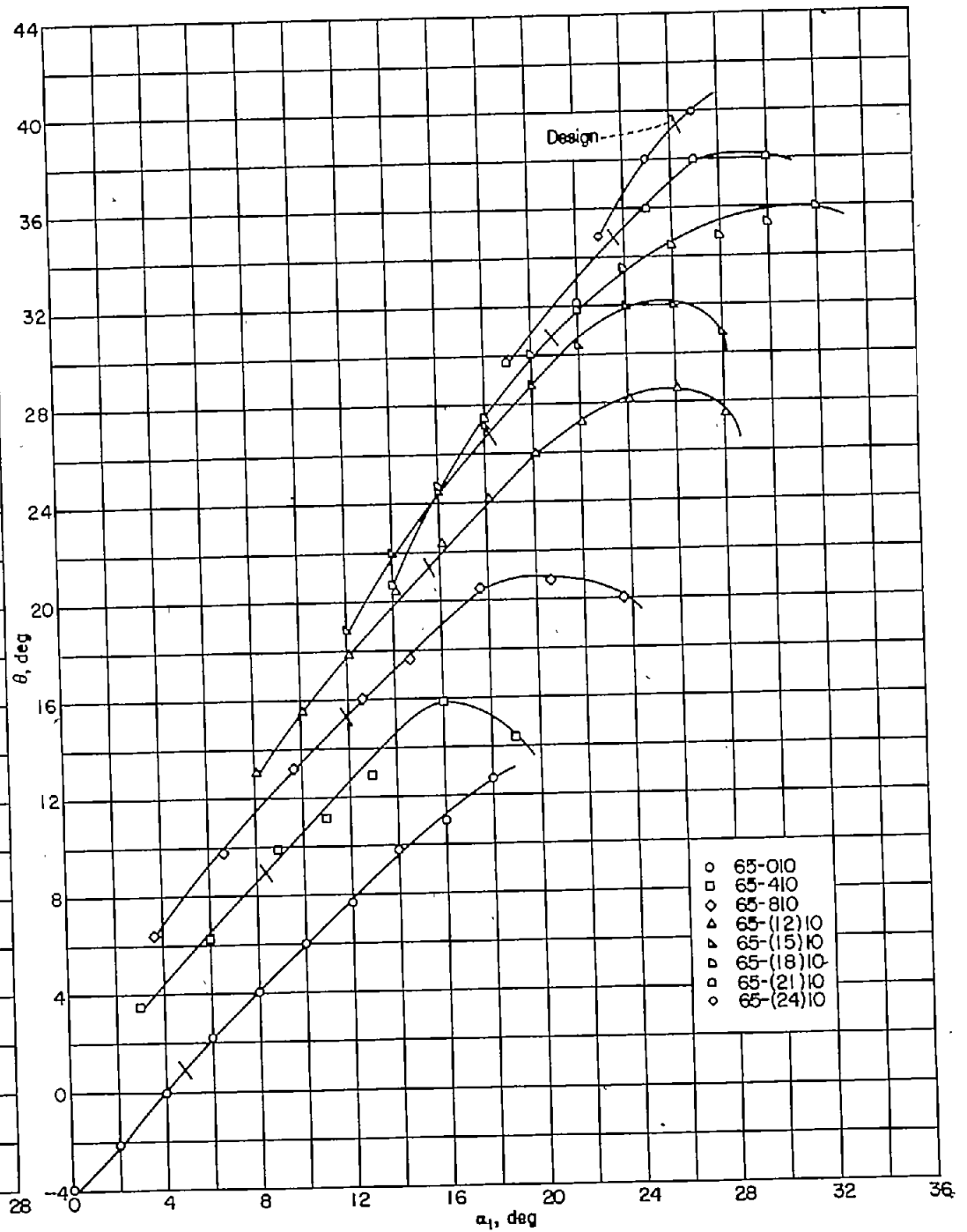
FIGURE 103.—Summary of relationship between turning angle \theta and angle of attack \alpha_1 for the blade sections tested at \beta_1=60^\circ , \sigma=1.50 .
