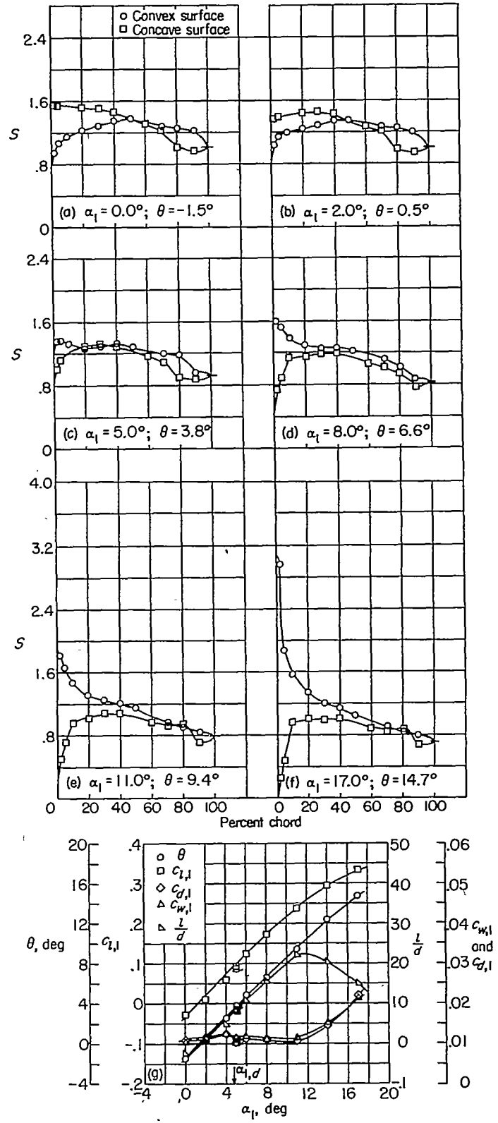
FIGURE 39.—Blade-surface pressure distributions and blade section characteristics for the cascade combination, \beta_1=45^\circ , \sigma=1.50 , and blade section, NACA 65-010.
