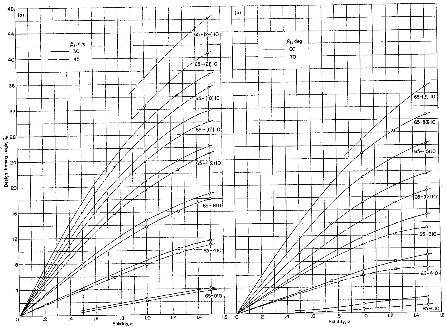
(b) Inlet angles of 60° and 70°.
