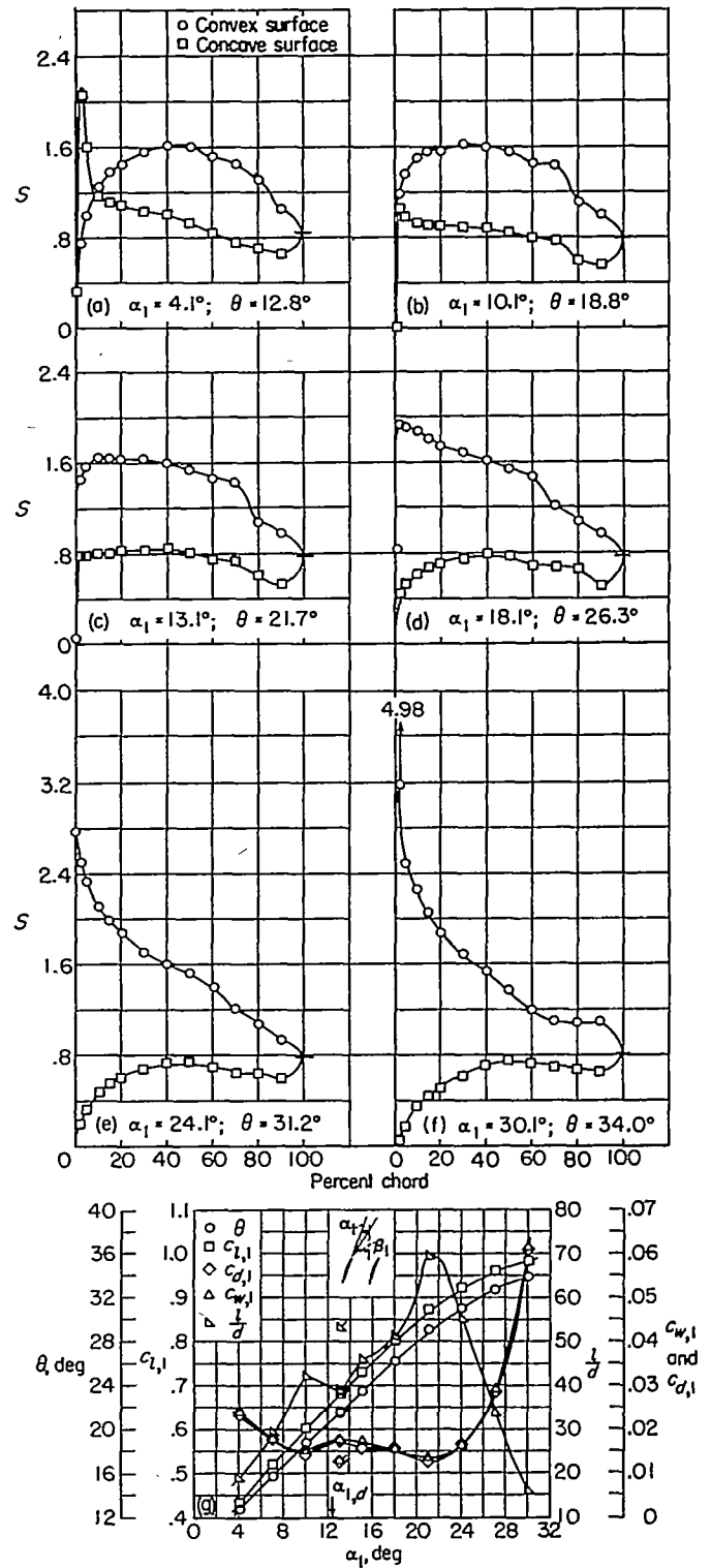
(g) Section characteristics; flagged symbol indicates leading-edge roughness.
