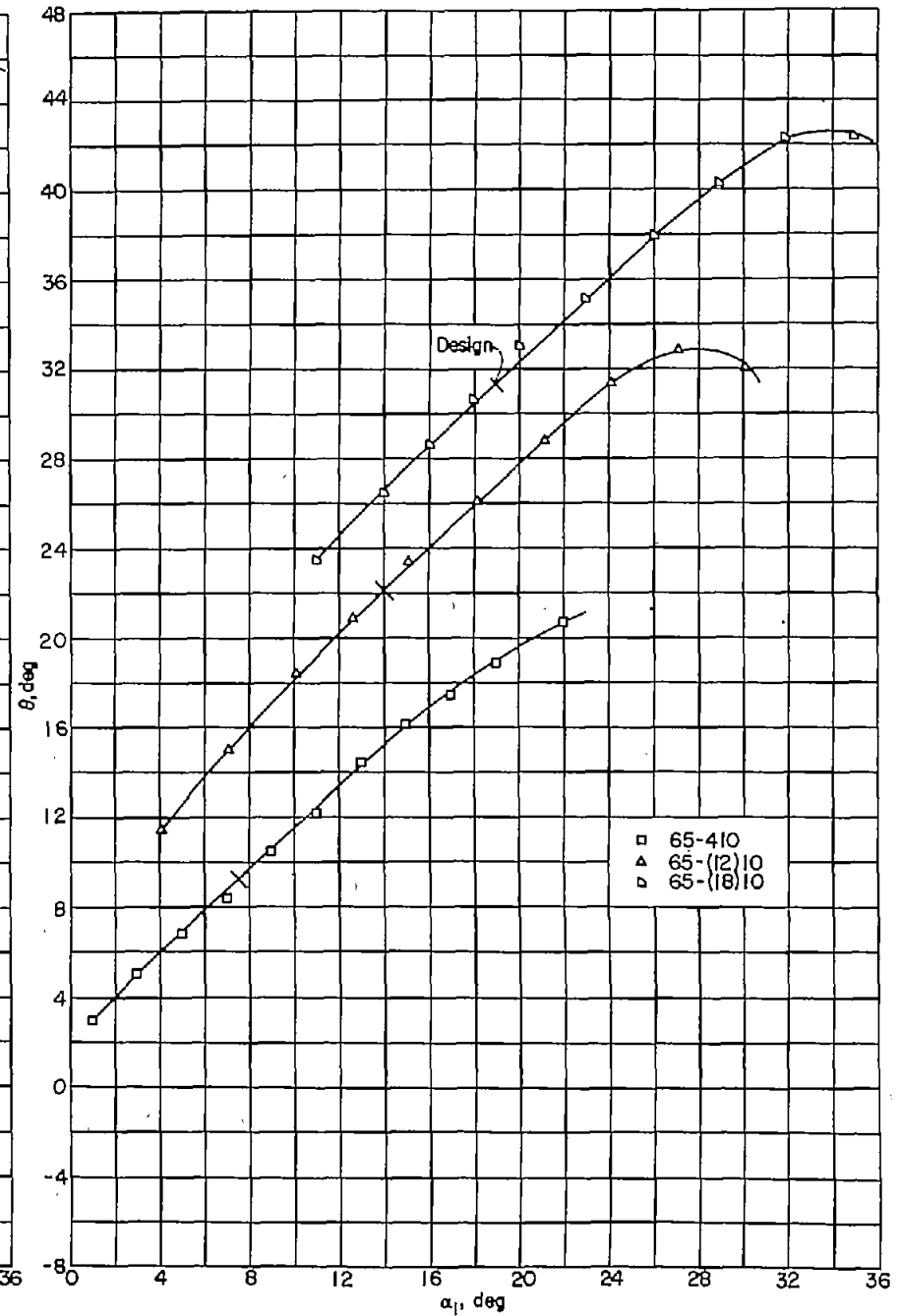
FIGURE 97.—Summary of relationship between turning angle \theta and angle of attack \alpha_1 for the blade sections tested at \beta_1=45^\circ , \sigma=1.25 .
