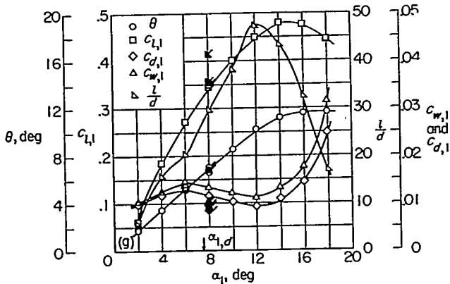
(g) Section characteristics; flagged symbol indicates leading-edge roughness; solid symbol indicates high Reynolds number.
