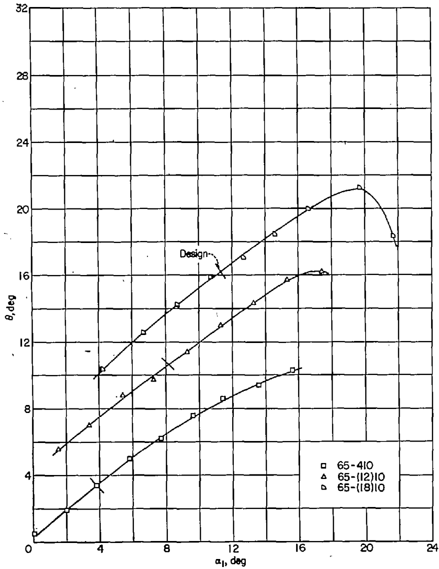
FIGURE 94.—Summary of relationship between turning angle \theta and angle of attack \alpha_1 for the blade sections tested at \beta_1=45^\circ , \sigma=0.50 .
