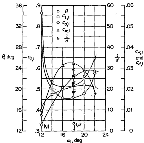
(g) Section characteristics; flagged symbol indicates leading-edge roughness; solid symbol indicates high Reynolds number.
