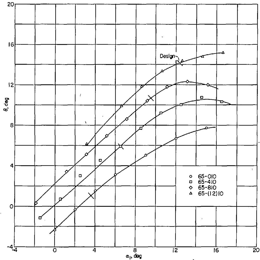
FIGURE 104.—Summary of relationship between turning angle \theta and angle of attack \alpha_1 for the blade sections tested at \beta_1=70^\circ , \sigma=1.00 .
