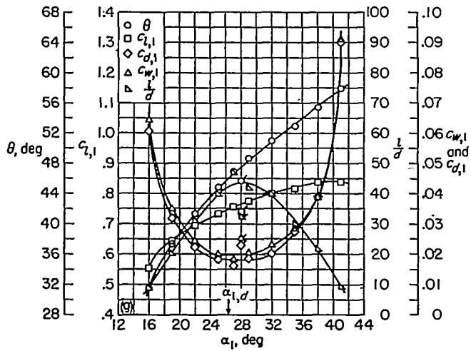
(g) Section characteristics; flagged symbol indicates leading-edge roughness. FIGURE 46.—Blade-surface pressure distributions and blade section characteristics for the cascade combination, \beta_1=45^\circ , \sigma=1.50 , and blade section, NACA 65-(24)10.
