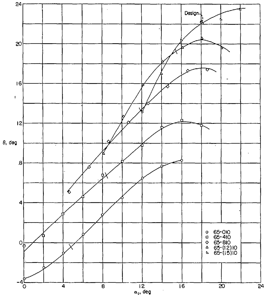
FIGURE 106.—Summary of relationship between turning angle \theta and angle of attack \alpha_1 for the blade sections tested at \beta_1=70^\circ , \sigma=1.50 .
