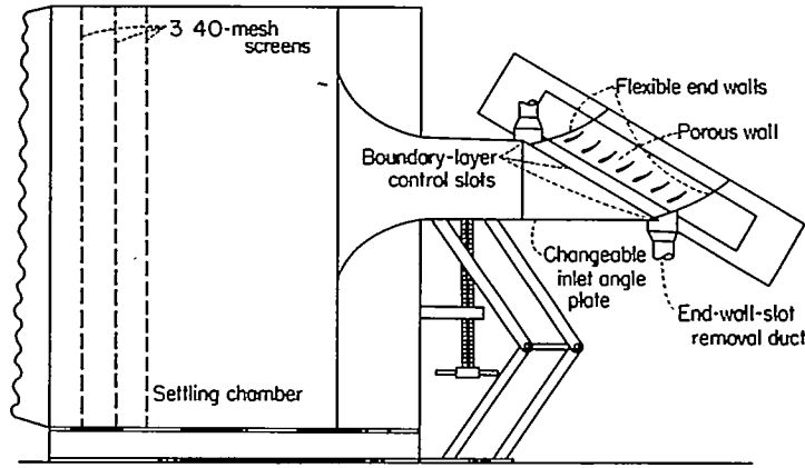
FIGURE 1.—Vertical cross section of two-dimensional low-speed cascade tunnel.
