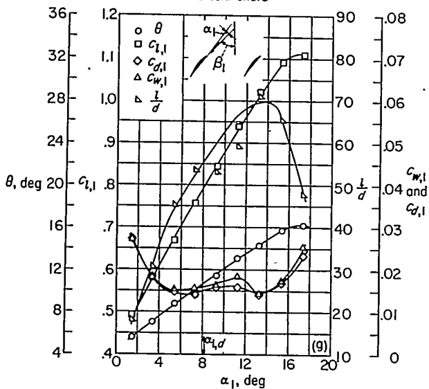
FIGURE 22.—Blade-surface pressure distributions and blade section characteristics for the cascade combination, \beta_1=45^\circ , \sigma=0.50 , and blade section, NACA 65-(12)10.
