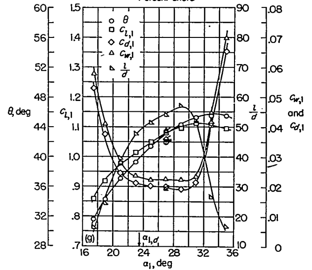
FIGURE 35.—Blade-surface pressure distributions and blade section characteristics for the cascade combination, \beta_1=45^\circ , \sigma=1.00 , and blade section, NACA 65-(27)10.
