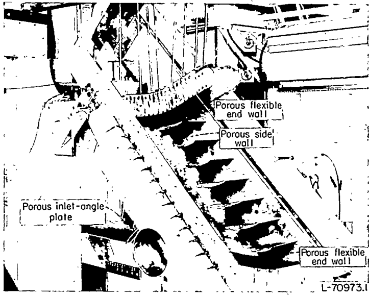
FIGURE 2.—Photograph of Langley 5-inch cascade tunnel with portions of one side removed to show porous surfaces.
