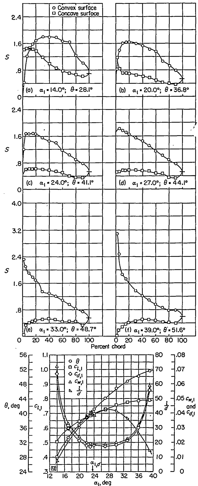
(g) Section characteristics; flagged symbol indicates leading-edge roughness.
