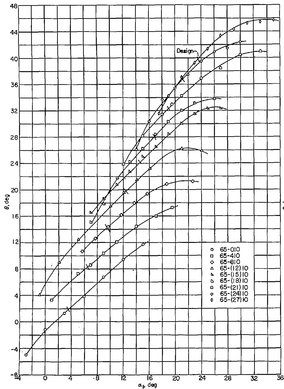
FIGURE 96.—Summary of relationship between turning angle \theta and angle of attack \alpha_1 for the blade sections tested at \beta_1=45^\circ , \sigma=1.00 .
