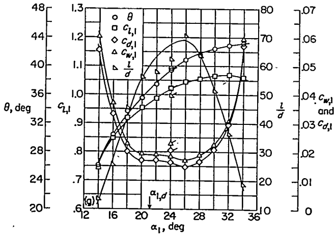
FIGURE 34.—Blade-surface pressure distributions and blade section characteristics for the cascade combination, \beta_1=45^\circ , \sigma=1.00 , and blade section, NACA 65-(24)10.
