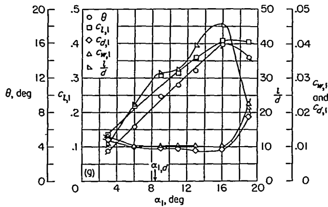
(g) Section characteristics.
