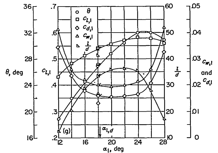
FIGURE 67.—Blade-surface pressure distributions and blade section characteristics for the cascade combination, \beta_1=60^\circ , \sigma=1.50 , and blade section, NACA 65-(15)10.
