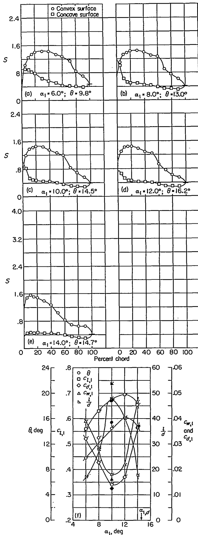
(f) Section characteristics; no design point was obtained; flagged symbol indicates leading-edge roughness; solid symbol indicates high Reynolds number.
