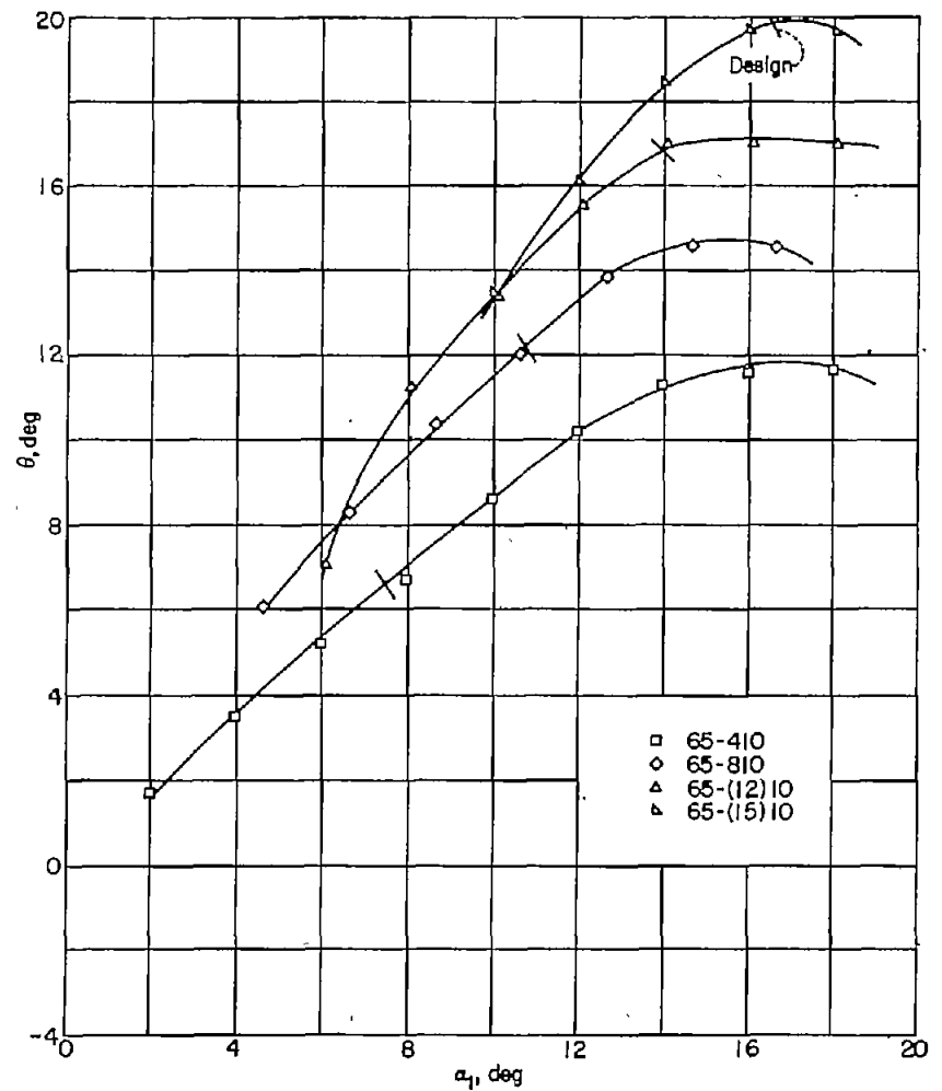
FIGURE 105.—Summary of relationship between turning angle \theta and angle of attack \alpha_1 for the blade sections tested at \beta_1=70^\circ , \sigma=1.25 .
