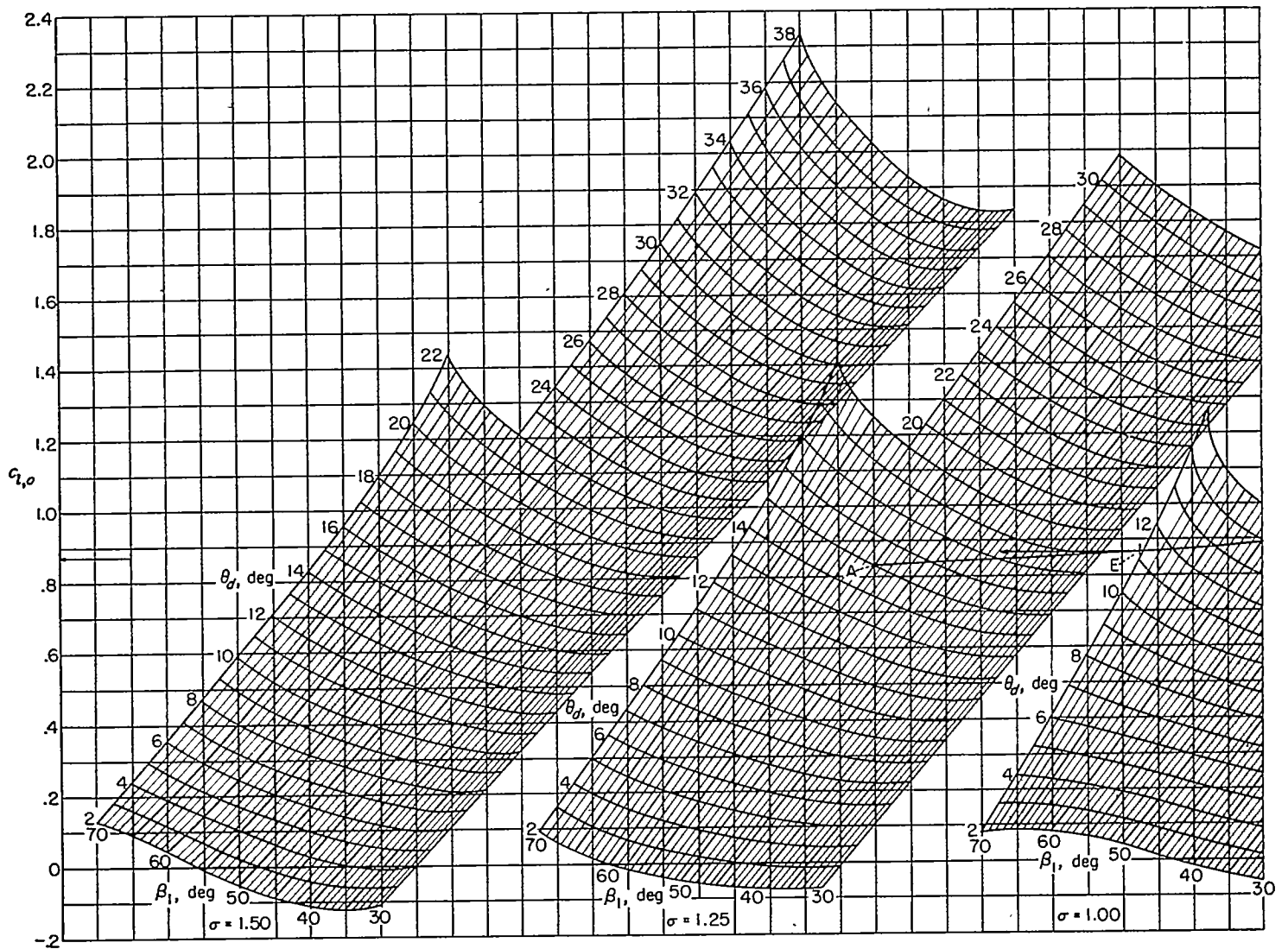
FIGURE 112.—Design-camber selection chart for NACA 65- (c_{l,o}) 10 sections.
