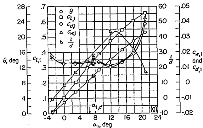
FIGURE 7.—Blade-surface pressure distributions and blade section characteristics for the cascade combination, \beta_1=30^\circ , \sigma=1.00 , and blade section, NACA 65-410.
