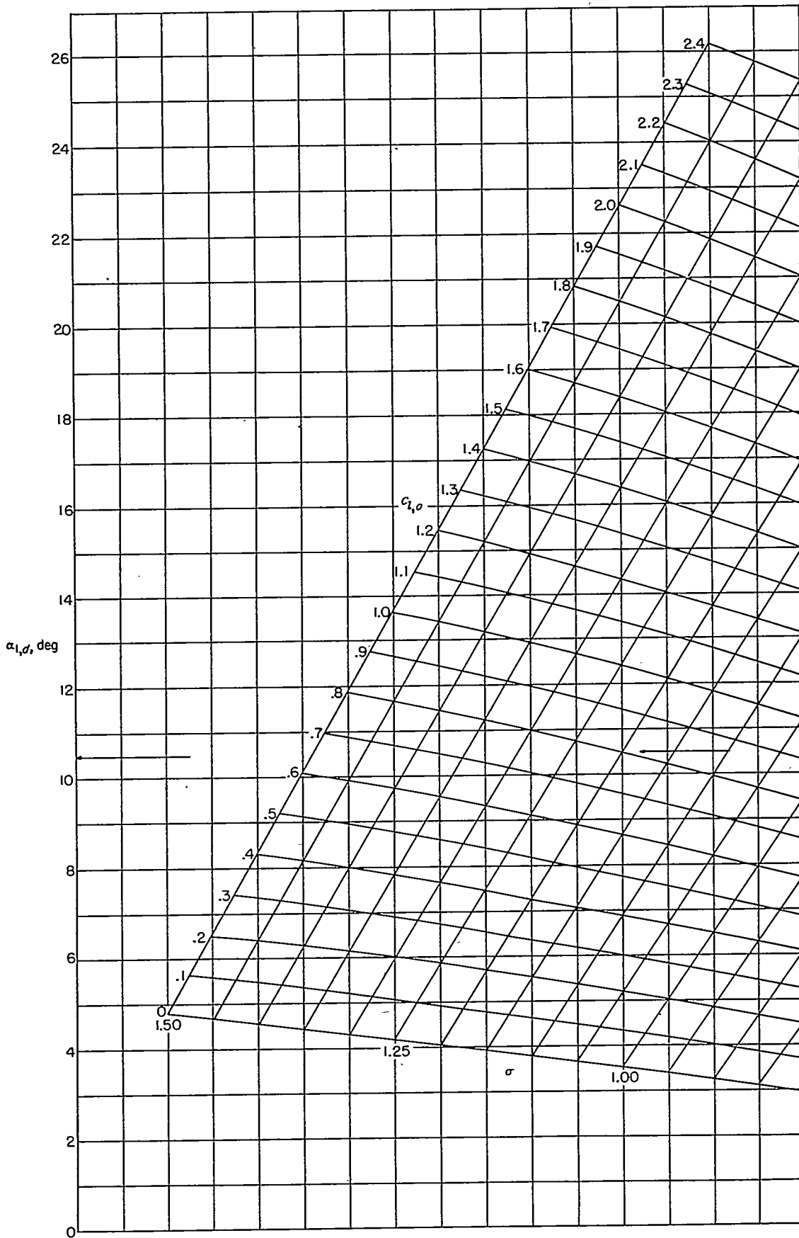
FIGURE 113.—Design angle-of-attack chart for NACA 65-( c_{l,\sigma} )10 sections.
