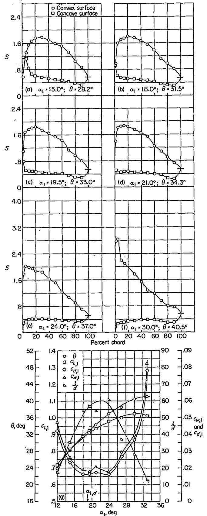
(g) Section characteristics.
