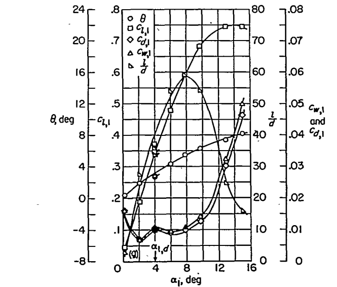
(g) Section characteristics; flagged symbol indicates leading-edge roughness. FIGURE 47.—Blade-surface pressure distributions and blade section characteristics for the cascade combination, \beta_1=60^\circ , \sigma=0.50 , and blade section, NACA 65-410.
