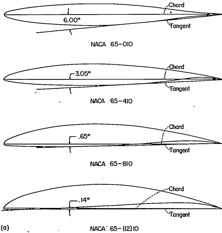
(a) Lower cambered sections. Angle between chord line and tangent to lower surface as shown for the various sections.
