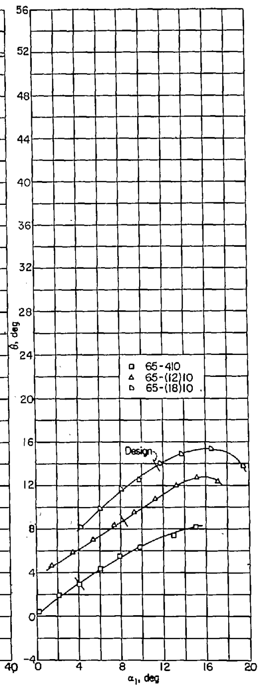
FIGURE 99.—Summary of relationship between turning angle \theta and angle of attack \alpha_1 for the blade sections tested at \beta_1=80^\circ , \sigma=0.50 .
