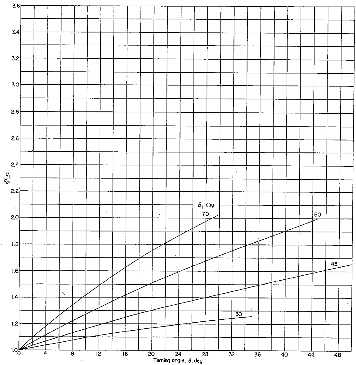
FIGURE 88.—Conversion chart showing the relation between entering and mean dynamic pressure as a function of turning angle and inlet angle.
