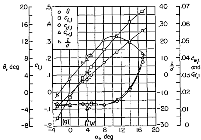
FIGURE 6.—Blade-surface pressure distributions and blade section characteristics for the cascade combination, \beta_1=30^\circ , \sigma=1.00 , and blade section, NACA 65-010.
