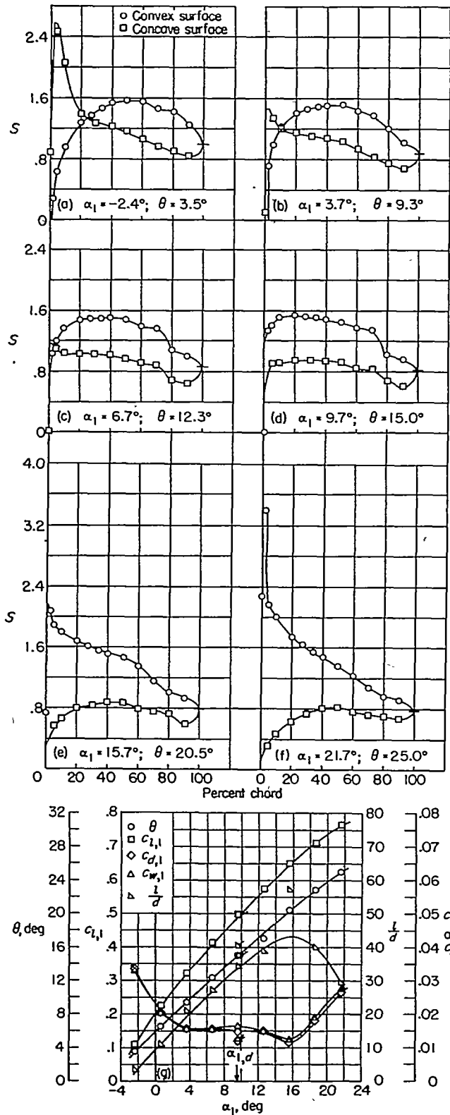
FIGURE 8.—Blade-surface pressure distributions and blade section characteristics for the cascade combination, \beta_1=30^\circ , \sigma=1.00 , and blade section, NACA 65-810.
