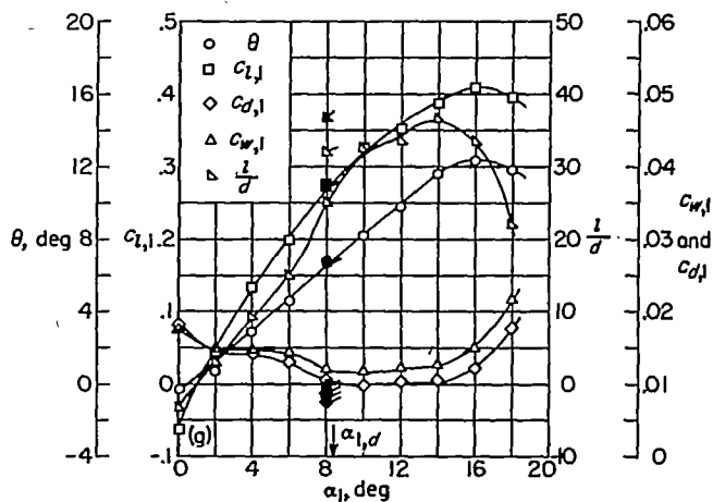
(g) Section characteristics; flagged symbol indicates leading-edge roughness; solid symbol indicates high Reynolds number.
