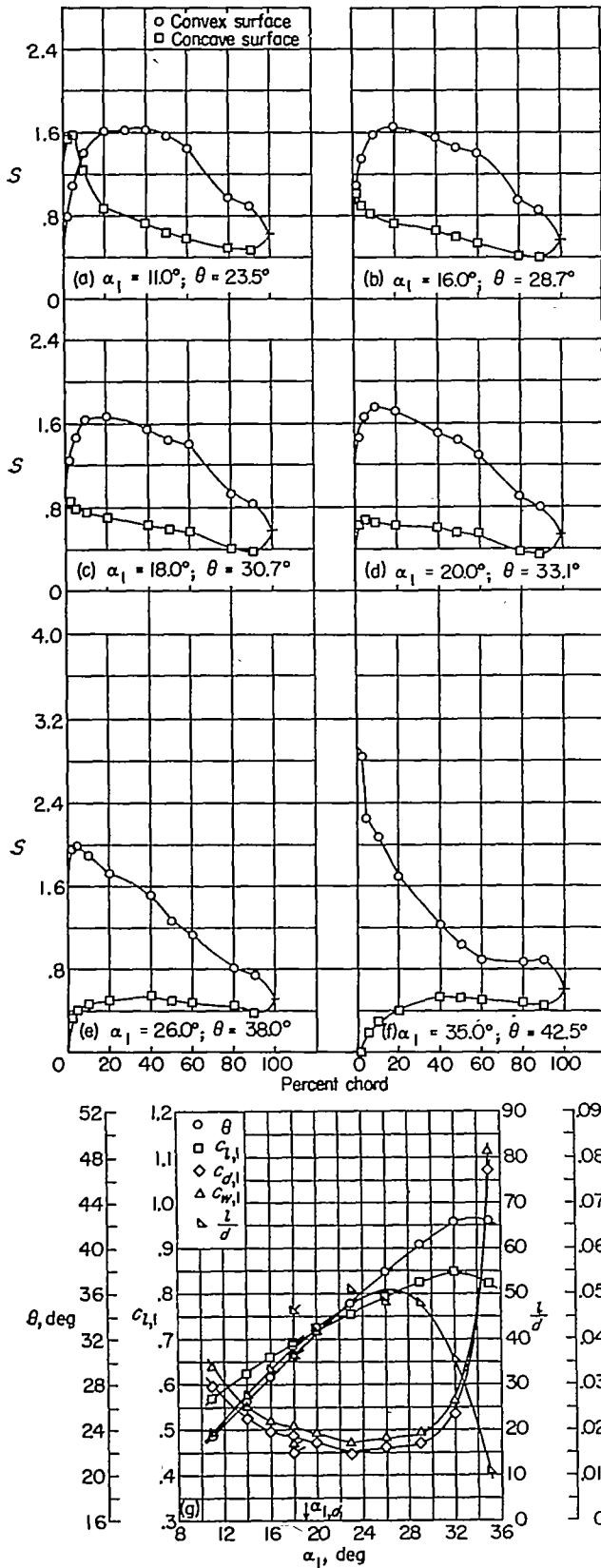
FIGURE 38.—Blade-surface pressure distributions and blade section characteristics for the cascade combination, \beta_1=45^\circ , \sigma=1.25 , and blade section, NACA 65-(18)10.
