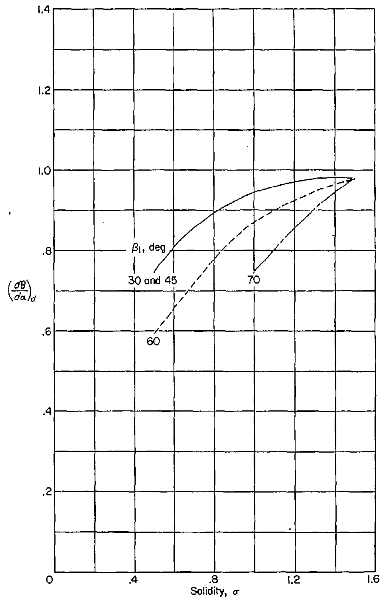
FIGURE 107.—Variation of slope of curves of turning angle against angle of attack at design conditions with solidity and inlet angle. The slopes are averages for the moderate camber range.
