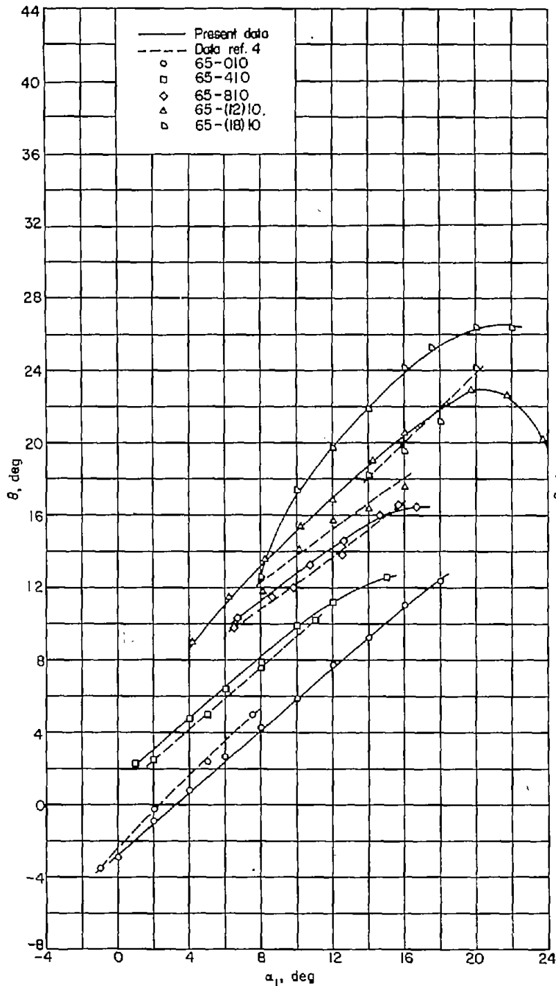
FIGURE 90.—Comparison of relationships between turning angle and angle of attack for the present porous-wall cascade results with those for the solid-wall cascade of reference 4 for a typical combination. \beta_1=60^\circ ; \sigma=1.00 .
