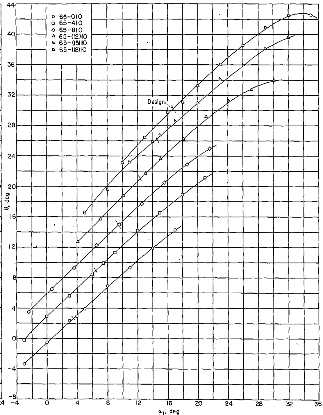
FIGURE 91.—Summary of relationship between turning angle \theta and angle of attack \alpha_1 for the blade sections tested at \beta_1=30^\circ , \sigma=1.00 .
