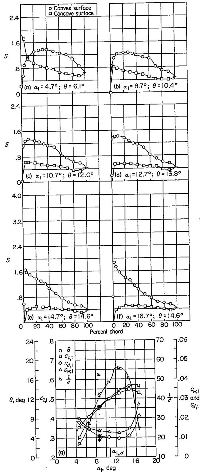
(g) Section characteristics; flagged symbol indicates leading-edge roughness; solid symbol indicates high Reynolds number.
