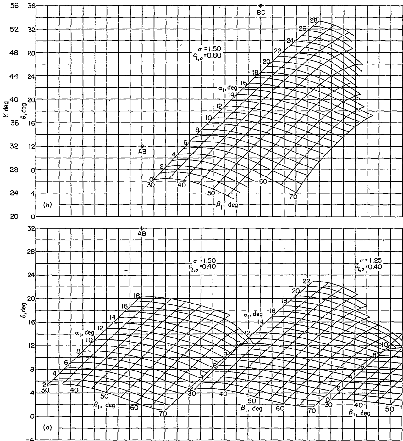
FIGURE 114.—Off-design turning-angle carpets for NACA 65-( c_{l,\sigma} )10 compressor blades.
