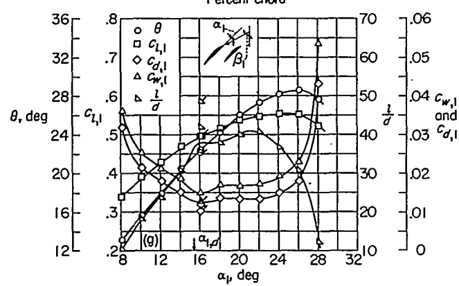
FIGURE 66.—Blade-surface pressure distributions and blade section characteristics for the cascade combination, \beta_1=60^\circ , \sigma=1.50 , and blade section, NACA 65-(12)10.
