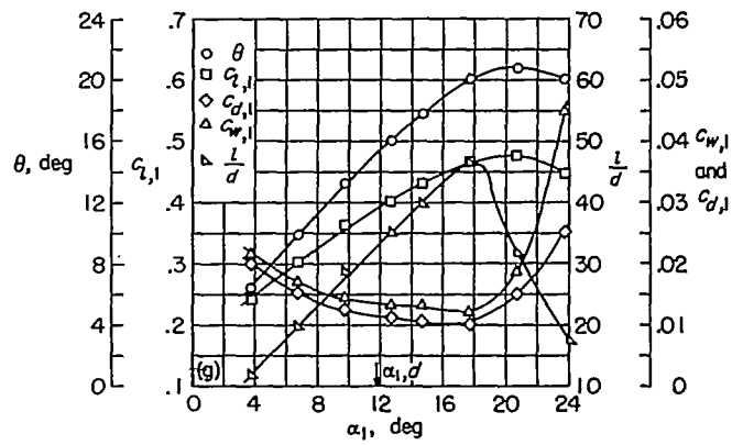
(g) Section characteristics.
