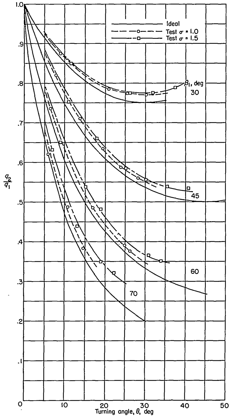
FIGURE 87.—Variation of ideal and test dynamic-pressure ratio across the cascade.
