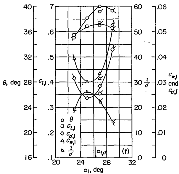
(f) Section characteristics; flagged symbol indicates leading-edge roughness.
