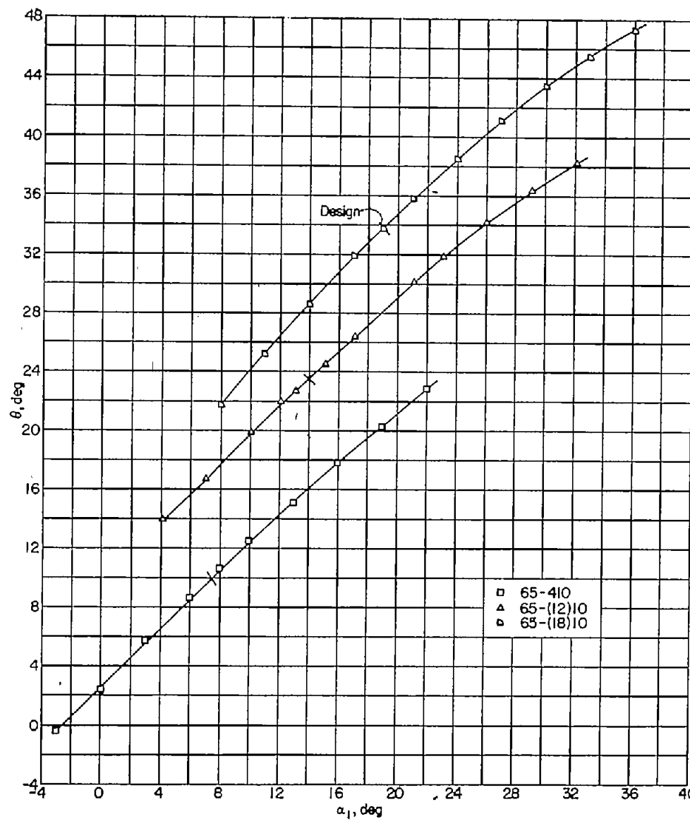
FIGURE 92.—Summary of relationship between turning angle \theta and angle of attack \alpha_1 for the blade sections tested at \beta_1=30^\circ , \sigma=1.25 .
