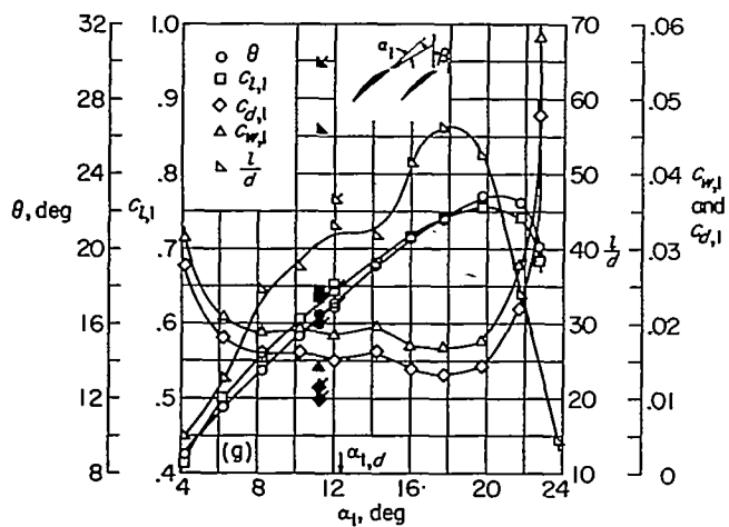
(g) Section characteristics; flagged symbol indicates leading-edge roughness; solid symbol indicates high Reynolds number.
