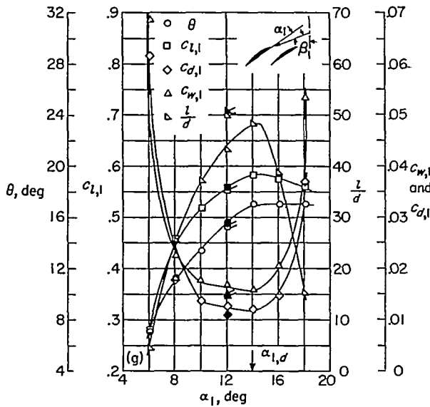
(g) Section characteristics; flagged symbol indicates leading-edge roughness; solid symbol indicates high Reynolds number.
