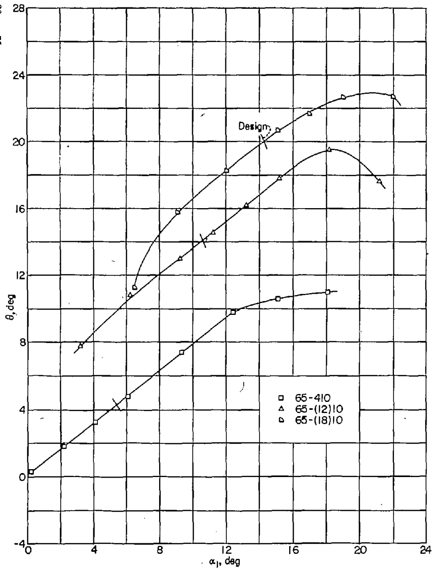
FIGURE 100.—Summary of relationship between turning angle \theta and angle of attack \alpha_1 for the blade sections tested at \beta_1 = 00^\circ , \sigma = 0.75 .
