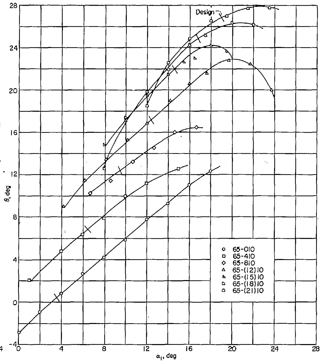
FIGURE 101.—Summary of relationship between turning angle \theta and angle of attack \alpha_1 for the blade sections tested at \beta_1 = 00^\circ , \sigma = 1.00 .
