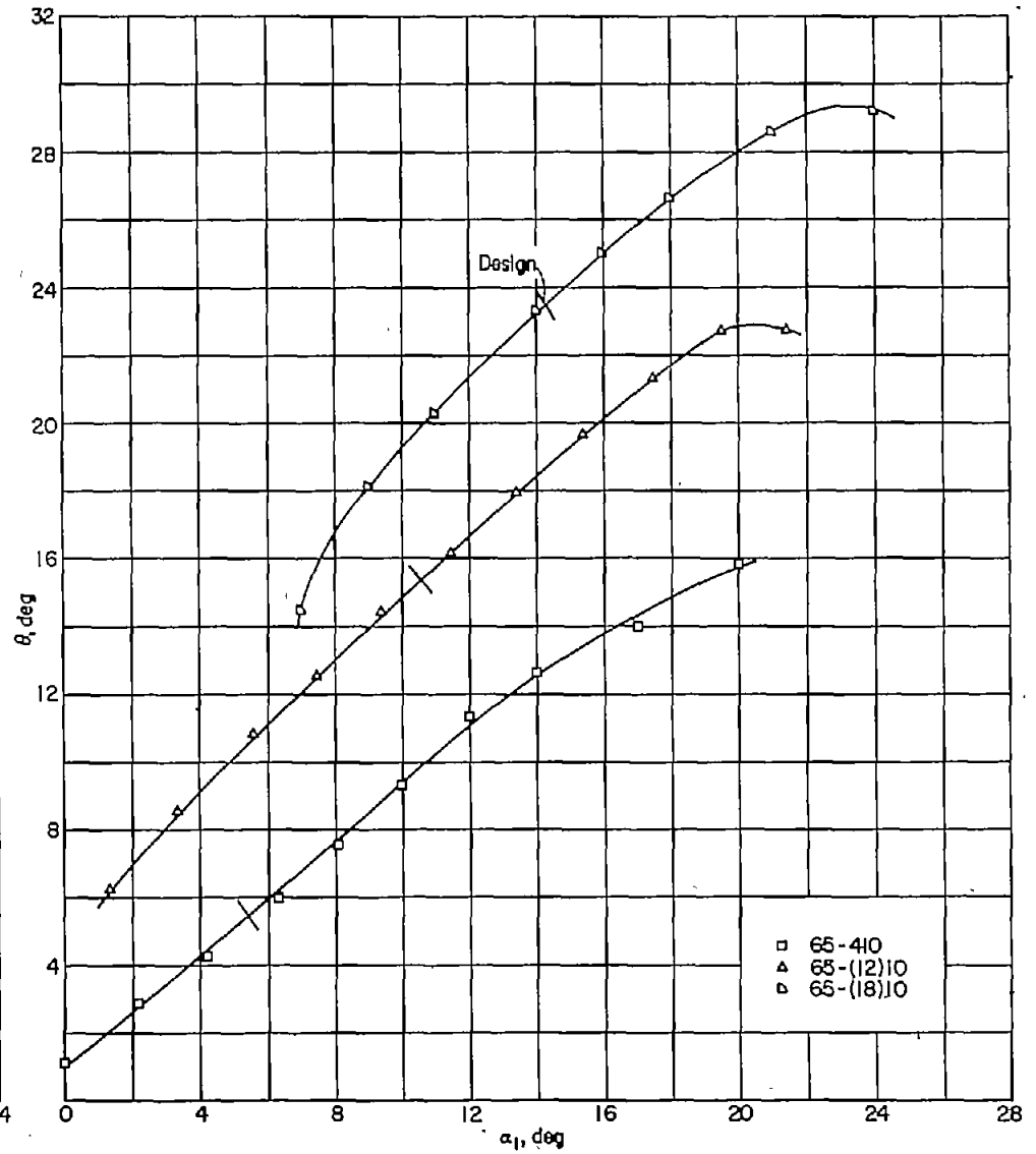
FIGURE 95.—Summary of relationship between turning angle \theta and angle of attack \alpha_1 for the blade sections tested at \beta_1=45^\circ , \sigma=0.76 .
