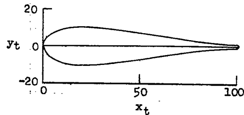
Thickness distribution coordinates t/c = 20 percent
