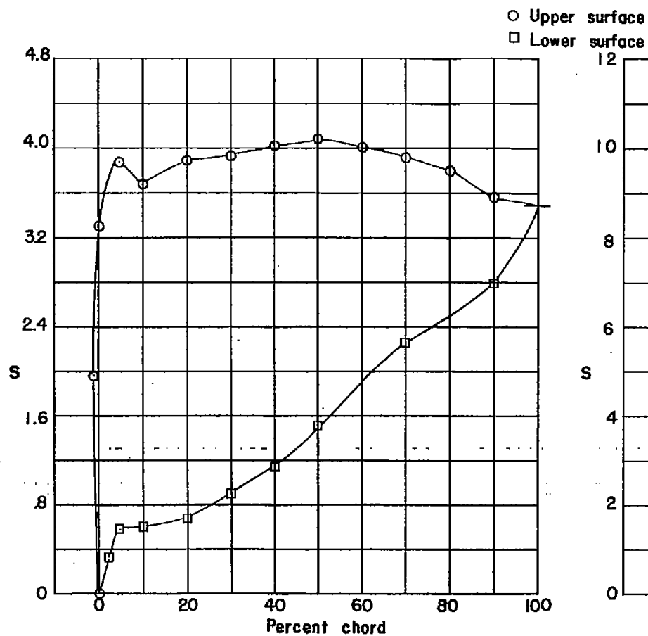
(a) M_1 = .289 ; M_2 = .56 ; C_{w_1} = .0202 ; \theta = 70.5^\circ .
