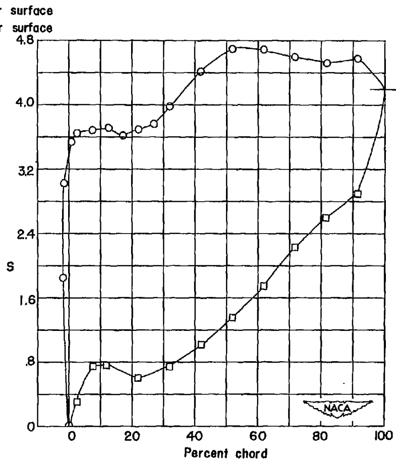
(b) M_1 = .362 ; M_2 = .813 ; C_{w_1} = .0212 ; \theta = 87.8^\circ
