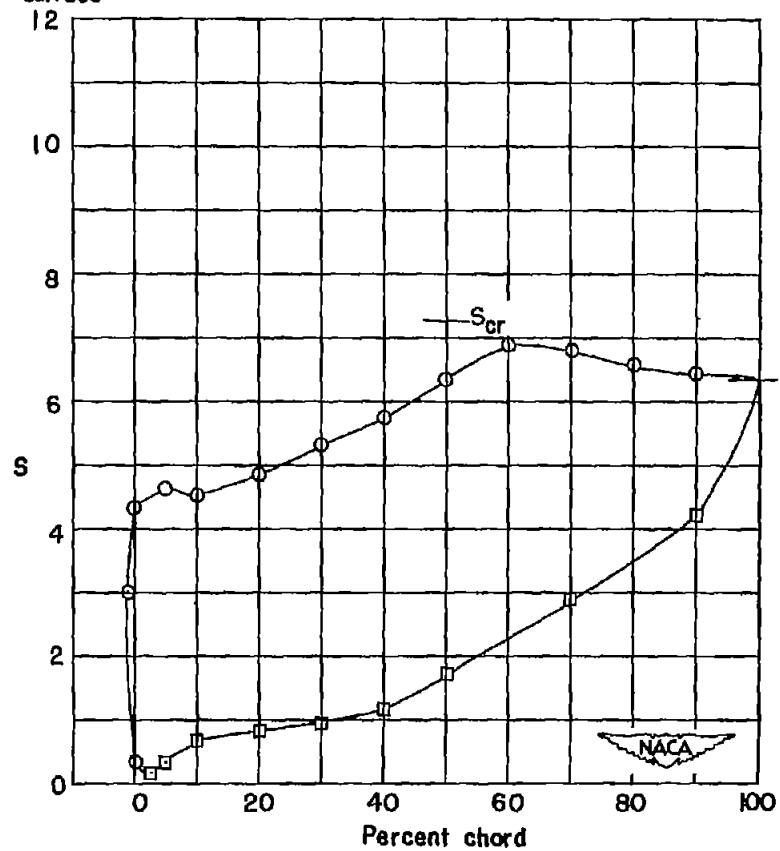
(b) M_1 = .315 ; M_2 = .908 ; C_{w_1} = .0231 ; \theta = 73.2^\circ .
