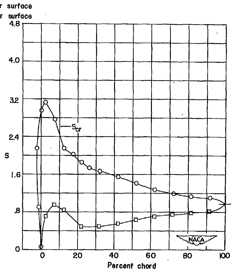
(b) M_1 = .566 ; M_2 = .539 ; C_{w1} = .0156 ; \theta = 85.1^\circ .
