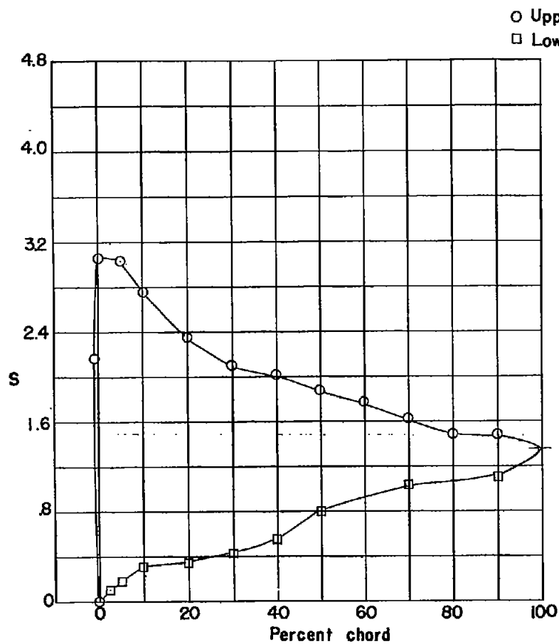
(a) M_1 = .265 ; M_2 = .330 ; C_{w1} = .0153 ; \theta = 73.4^\circ .
