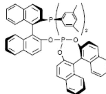
47 (R,S)
