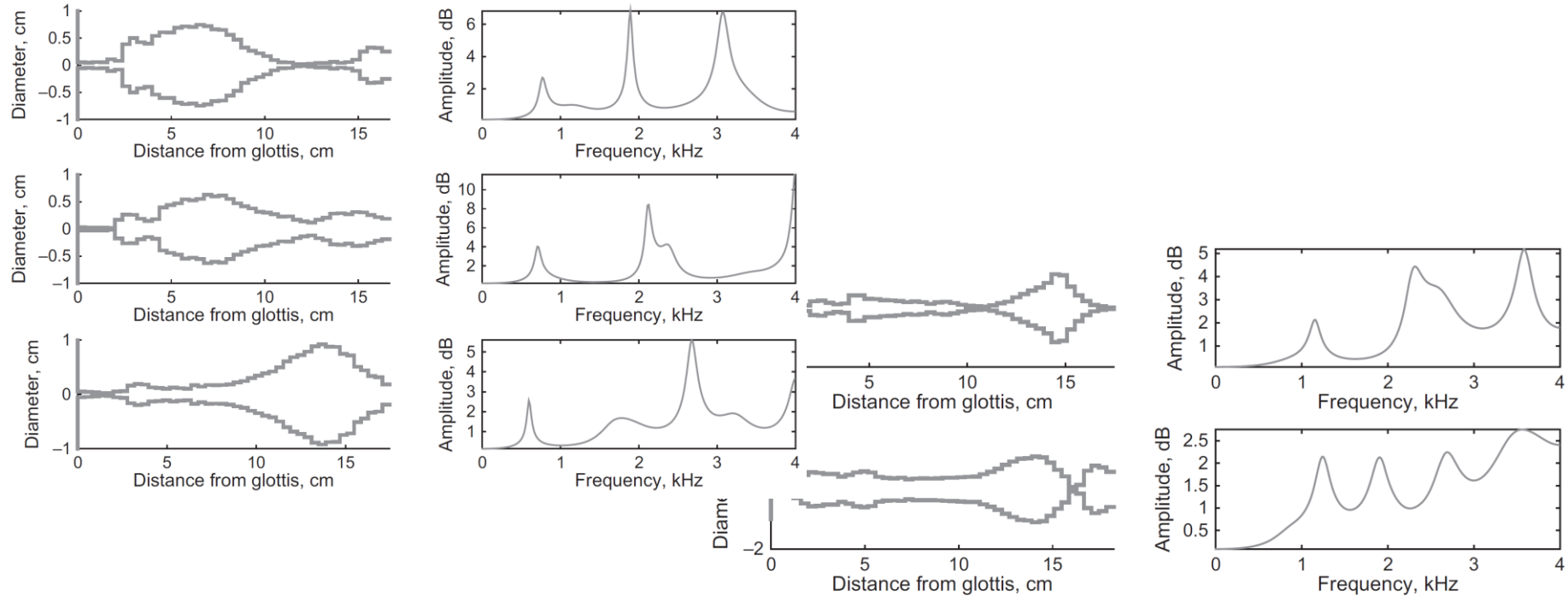
Figure 6.13 Tube cross-sections on the left, and frequency responses on the right for vowels /i/, /u/, /ɔ/, /o/ and consonant /l/ (all in IPA notation).
