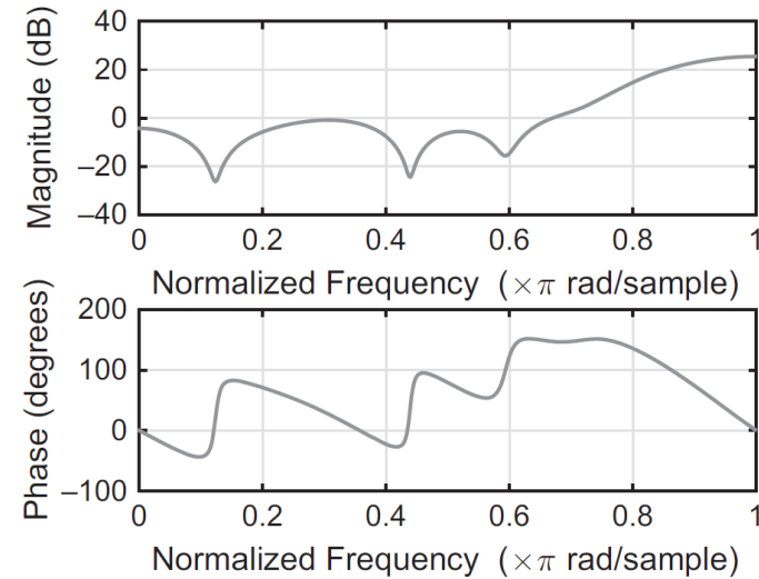
(b) \text{freqz}(a)
