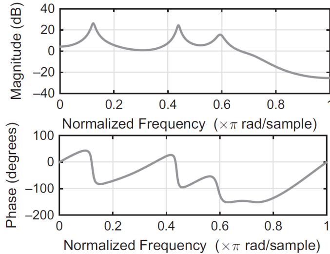
(a) \text{freqz}(1, a)
