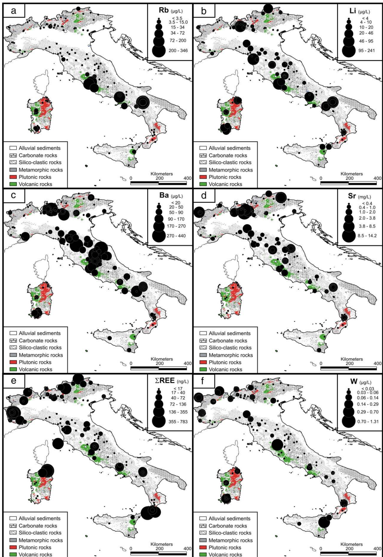
Fig. 6. Italian bottled waters dot maps of Rb (a), Li (b), Ba (c), Sr (d), \Sigma\text{REE} (e) and W (f).
