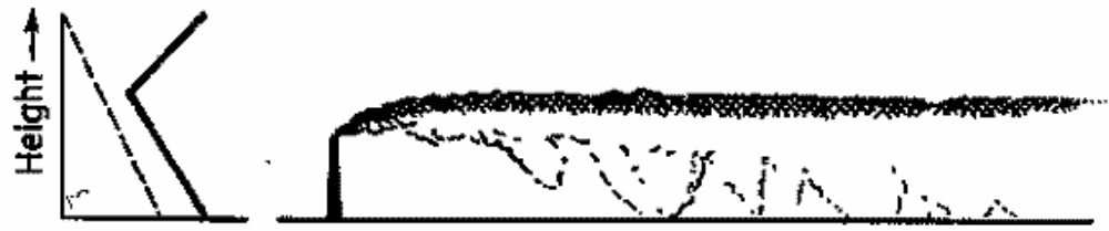
LAPSE BELOW, INVERSION ALOFT (FUMIGATION)
