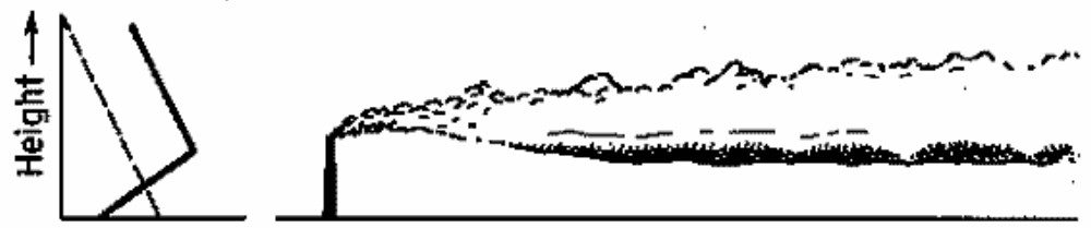
INVERSION BELOW, LAPSE ALOFT (LOFTING)
